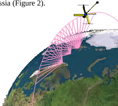
Figure 1: Geometry of the University of Wales radiotomography experiment in Scandinavia.
