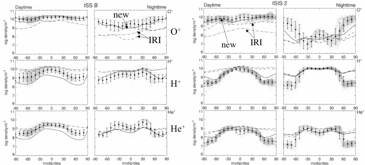
Figure 4. Daytime and nighttime latitudinal profiles of O^+ , H^+ , and He^+ densities during equinox as measured by ISS-b ( \bullet ) at 1000 km (left panel) and as predicted by the new IRI model (solid line) and by the earlier IRI standard (dashed line) and Danilov-Yaichnikov option (dash-dot line). The right panel shows a similar comparison for ISIS-2 at 1400 km also at equinox.
