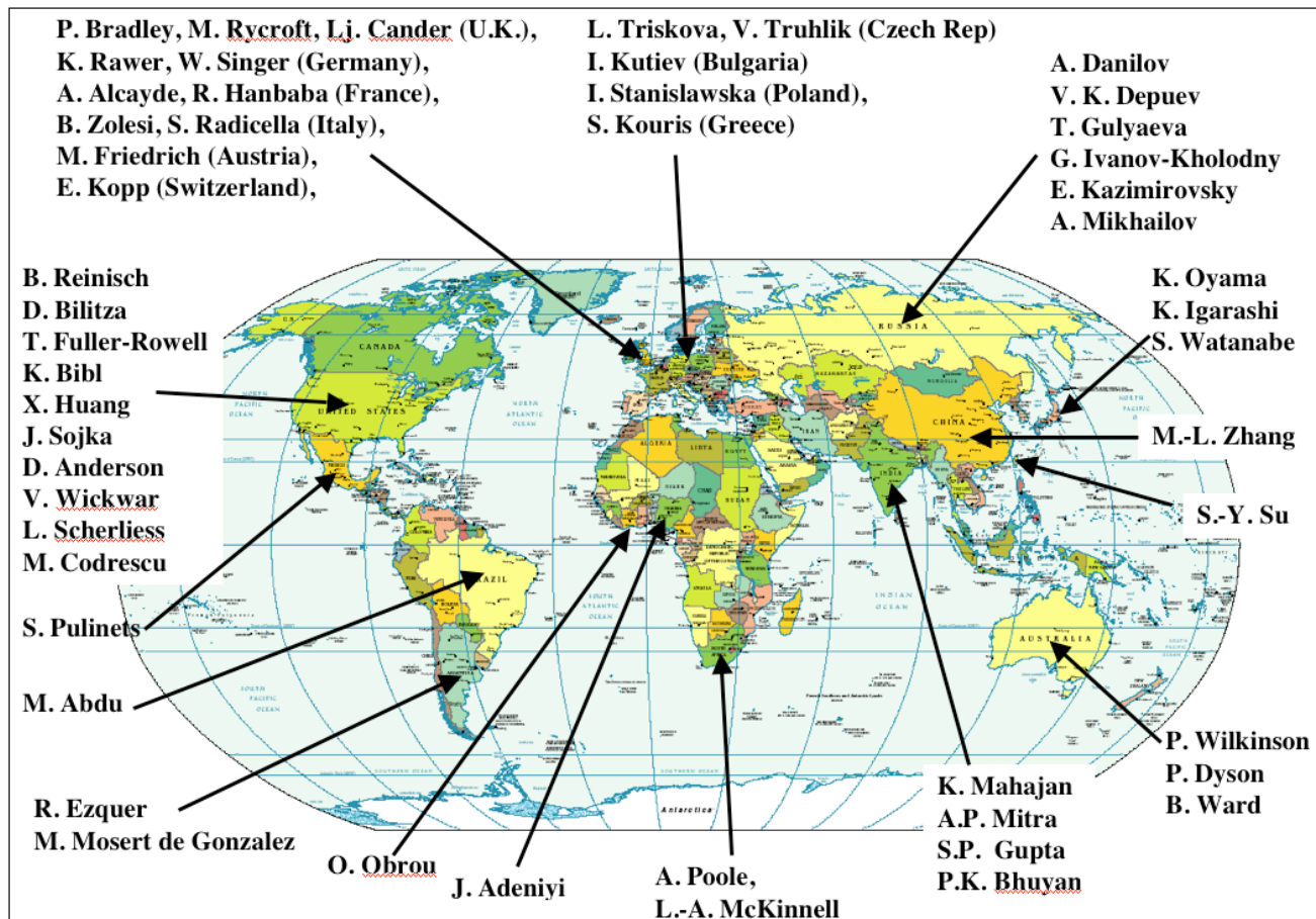
Figure 1: Global distribution of IRI Working Group members.
