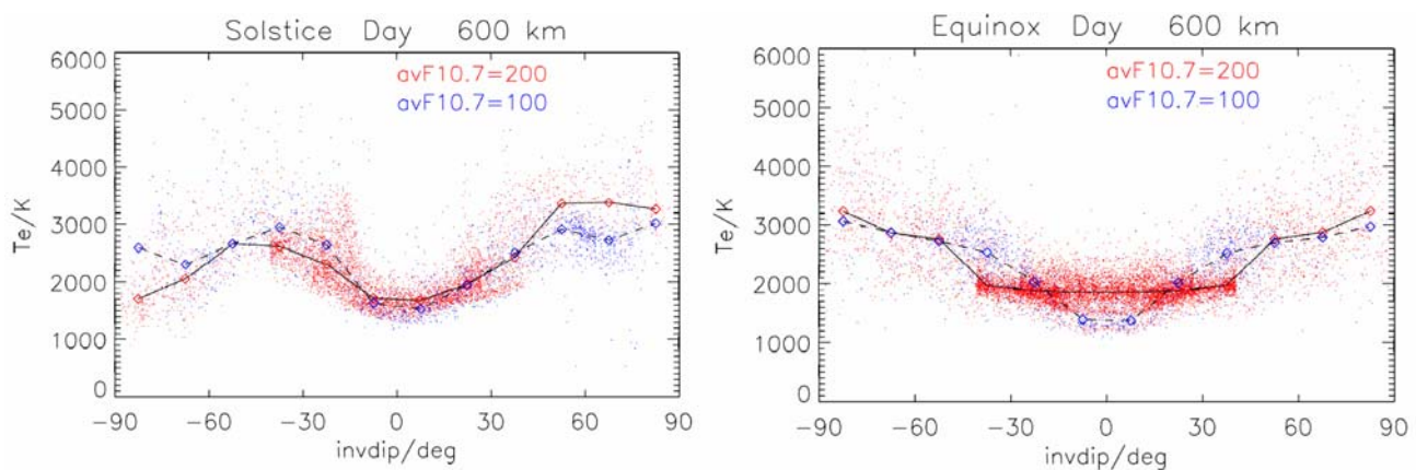
Figure 3. Electron temperature from satellite database versus dip latitude for high (red) and low (blue) solar activity and for summer solstice (left panel) and equinox (right panel); the special invdip latitude is used here which is close to the dip latitude at middle and low latitudes and close to invariant latitude at higher latitudes; the solar index is the solar radio flux at 10.7 cm wavelength.
