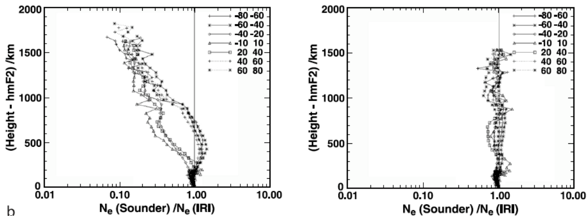
Figure 2 Average ratio between the Alouette/ISIS sounder data and the IRI model during noon for different modified dip latitude ranges using the current IRI topside model (left) and the corrected model (right). The model and data are normalized to the F-peak density and height.
