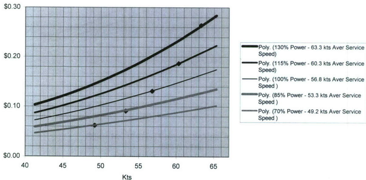
Figure No. 18 - Fuel Cost per PAX per nm @ $3.65/gal 500 nm Trip 105' lwl (125' oa) WarpDrive Fast Ferry
