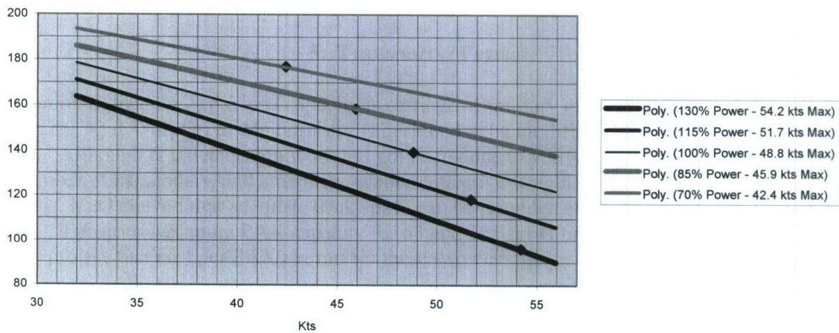
Figure No. 17 - Max PAX with Fuel for 500 nm 63' lwl (50' oa) WarpDrive Fast Ferry
