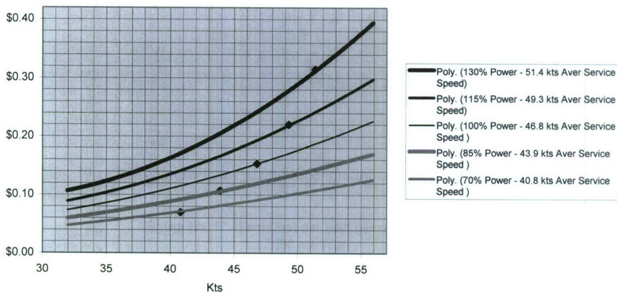
Figure No. 17 - Fuel Cost per PAX per nm @ $3.65/gal 500 nm Trip 63' lwl (75' oa) WarpDrive Fast Ferry
