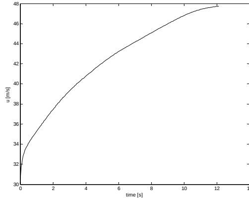
Figure 5.17: 5 Mountains – 6DoF – velocity u over time
