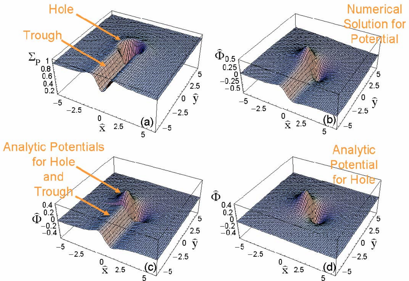
Figure 5. Electric potentials for a plasma bubble (a) formed by attached a plume to a circular density cavity. The numerical solution of the potential equation (b) is approximated by the analytic solutions of the potentials for the plume attached to the potential for the cavity (c). The potential fluctuations at the tip of the bubble closely match the analytic dipole potential (d) associated with the plasma hole.
