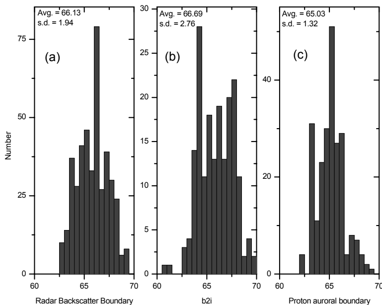
Figure 3: Distribution of the boundaries determined by (a) radar (b) DMSP satellite, and (c) H\beta emission.
