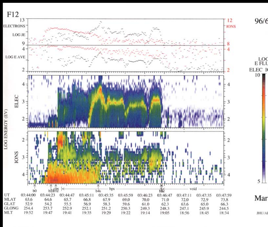
DMSP Particle Spectrogram
