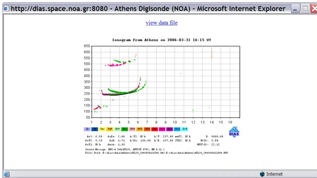
Figure 1: An ionogram from Athens Digisonde in DIAS layout. The results of the automatic scaling are also given. Clicking on the “View data file” the user can download the SAO file for the specific sounding.
