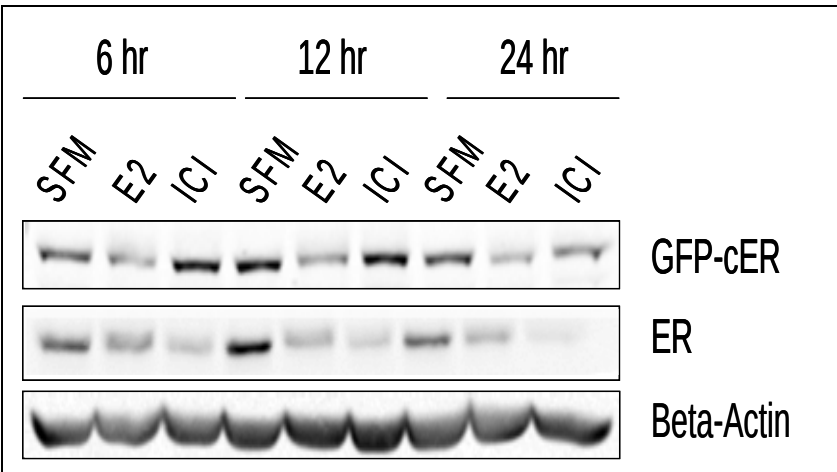
Figure 2. cER degradation by ICI is dependent on length of exposure to ligand. MCF-7-cER cells were starved in SFM overnight and then treated with either E2 ( 10^{-9} M) or ICI ( 10^{-9} M) for 6hr, 12hr, or 24hr. Protein levels were detected by Western blot, using antibodies against either ER \alpha or beta-actin.
