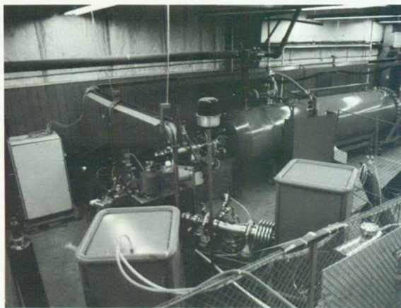
Positive Ion Accelerator at Manufacturer's Site.
