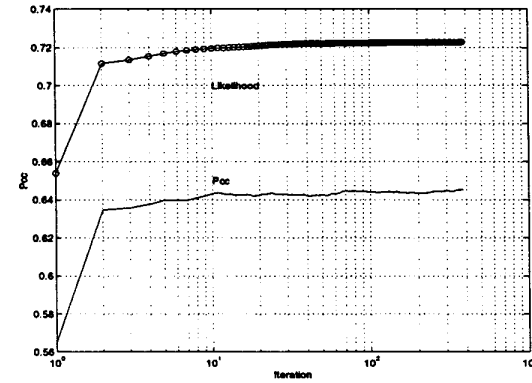
Figure 2: Repeat of Figure 1 with labeled data used to train p(Z_m|H_m) .
