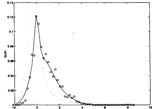
Figure 3: PDF estimation results for feature Z_4 using unlabeled data. Graph includes histogram of data from all 7 classes (dotted), histogram of data from class 4 (circles), PDF estimate for p(Z_4|H_4) (solid). Data is plotted on a normalized axis. The designation "SUX1" is the name used to identify feature Z_4 .
