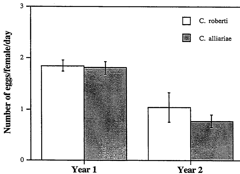
Fig. 4. Number of eggs/female/day laid during two separate oviposition periods of Ceutorhynchus roberti and C. alliariae . Data are means \pm SE of 7-10 replicates/ species/ year.
