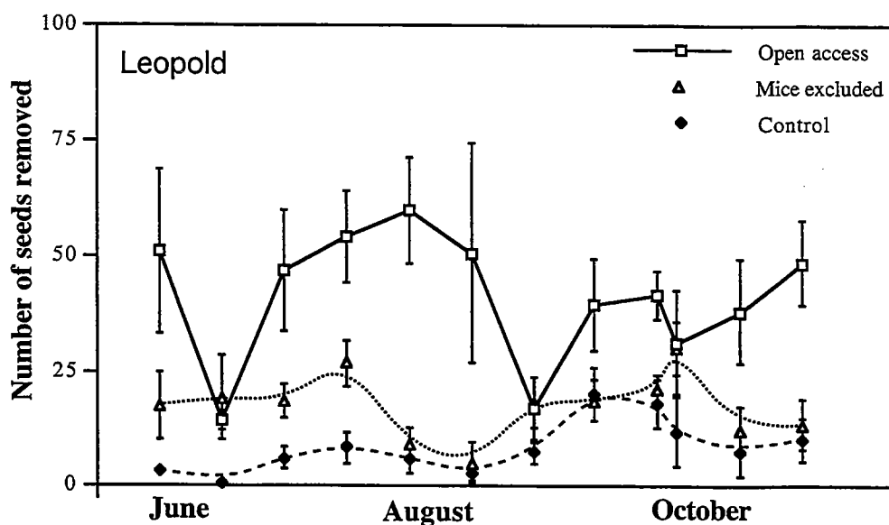
Fig. 48. Number of garlic mustard seeds removed in 14-day intervals during the 2001 field season from cages established in garlic mustard free areas at Leopold, Ithaca, NY. Solid lines represent cages allowing free access by seed predators, stippled lines represent cages where mice were excluded and dashed lines represent control (access by seed predators prevented). Data are means \pm SE of 5 replicates per treatment.
