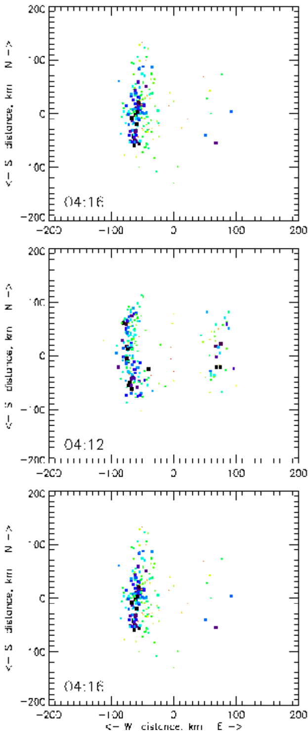
Figure 5: Skymaps of the auroral patch at 3 times.
