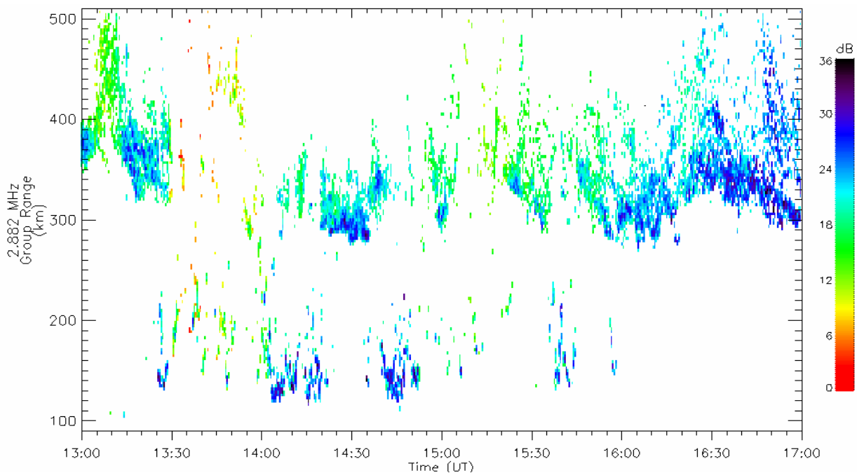
Figure 7: Example of poleward moving auroral forms for 1994 December 13 at Resolute Bay.
