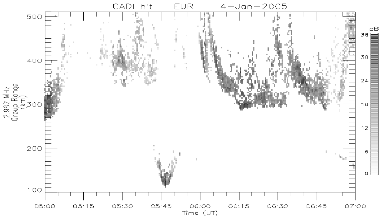
Figure 6: Distinctive V-shaped features due to rapidly moving auroras.
