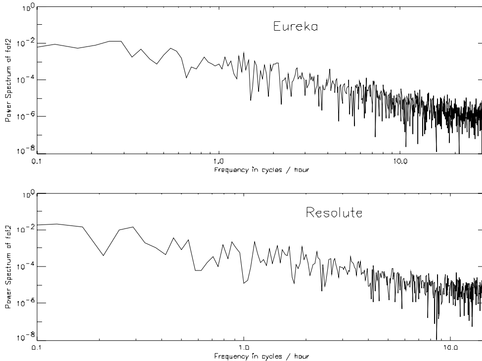
Figure 2: Power spectrum of the patches for 1996 March 3.
