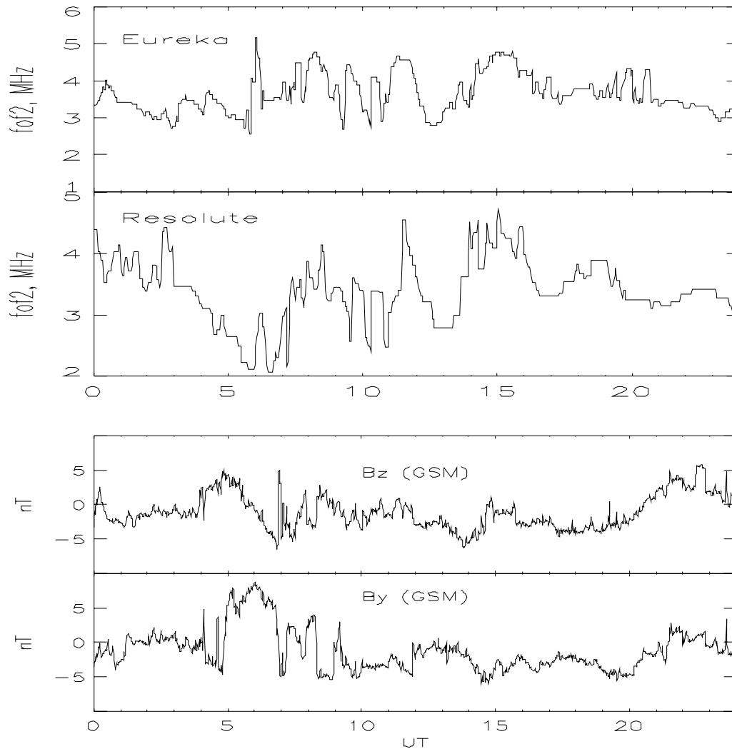
Figure 1: Data for 1996 March 3. The top panel shows f_o f_2 at Eureka and Resolute Bay. The bottom panel shows IMF data.
