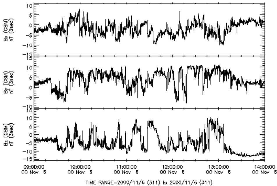
Figure 10: IMF data for the time interval in Figure 9. (Data from CDAWeb courtesy R. Lepping, NASA/GSFC)
