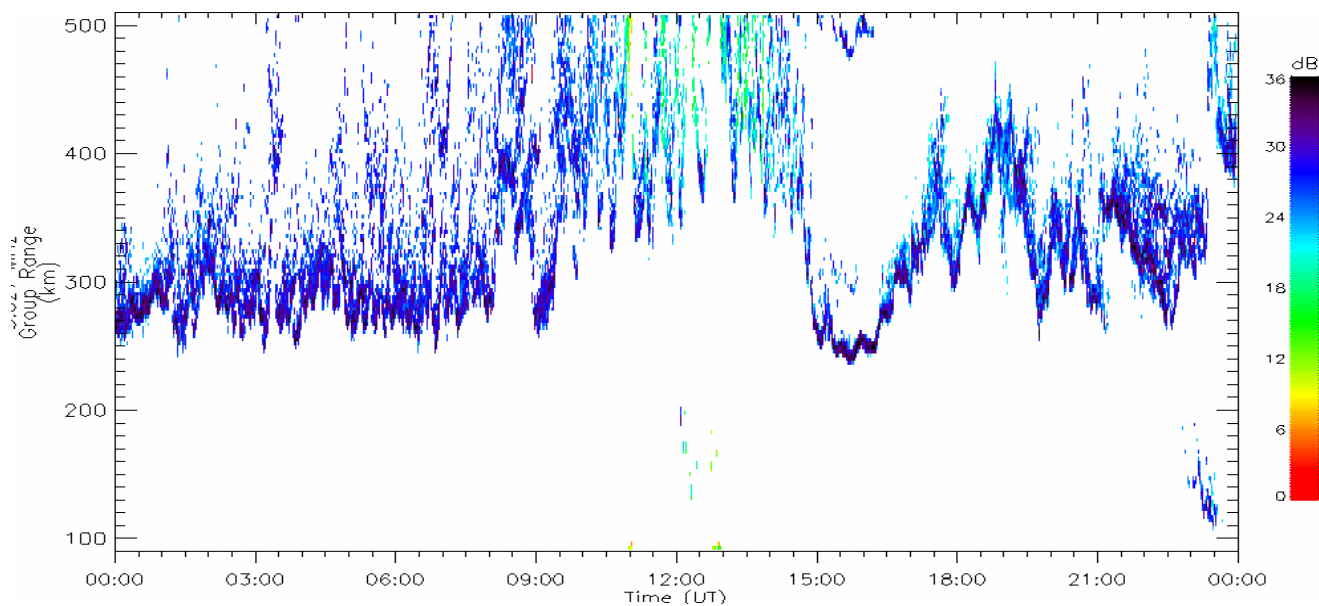
Figure 8: Height-time plot for 2000 November 6 on 3.027 MHz for Resolute Bay
