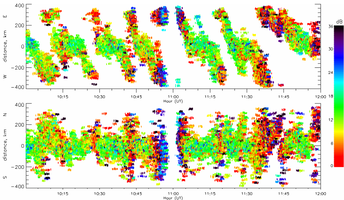
Figure 9: Horizontal location of echoes for the patches shown in Figure 8.
