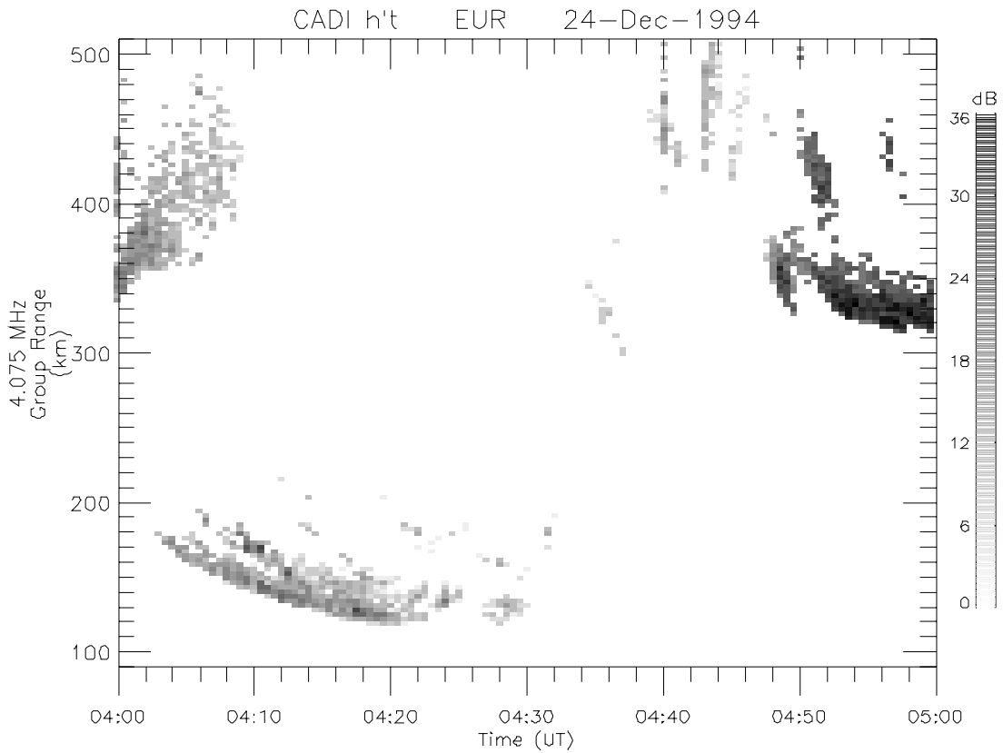
Figure 3: A polar cap aurora seen 1994 December 24 at Eureka. This shows the height-time at 4 MHz frequency.
