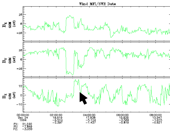
Figure 4: IMF during the Figure 3 event.
