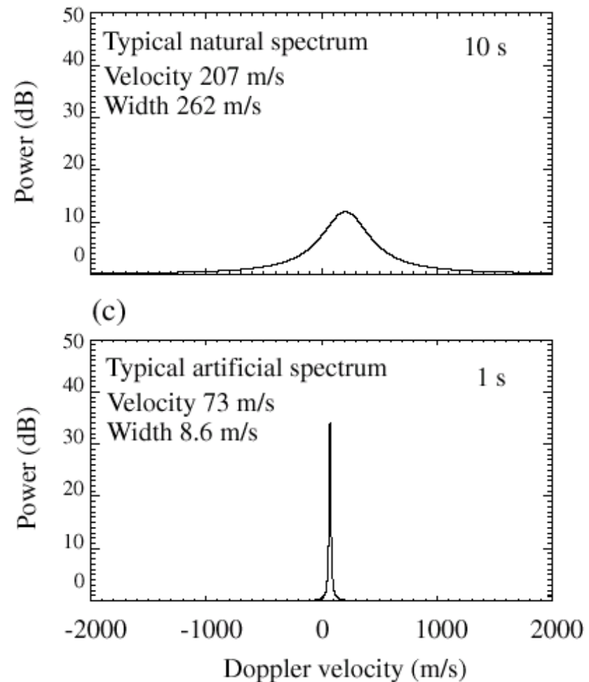
Fig. 1. (a) A schematic of the artificial backscatter experiment, SP-UK-OUCH. The Tromsø heater continuously heats the F region ionosphere, creating artificial ionospheric irregularities. These are detected by the CUTLASS radars, operating in a high temporal and spatial resolution mode. (b) A typical HF radar spectrum, obtained from fitting to the autocorrelation function of backscatter from natural F region irregularities after an integration period of 10 s. (c) A similar spectrum, but this time obtained from a 1 s integration from a heated F region. A narrower spectrum results, even from a shorter integration time.
