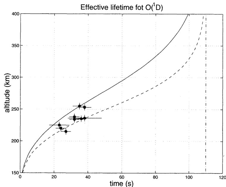
Figure 3: Altitude variation of the decay time constants of O(^1D) from [24]. The dot-dashed line shows the radiative lifetime of O(^1D) , the dashed curve including quenching by O_2 , N_2 and ambient electrons, the solid curve including quenching by atomic oxygen. The markers show estimates of the time constant from the experiment described in [21].
