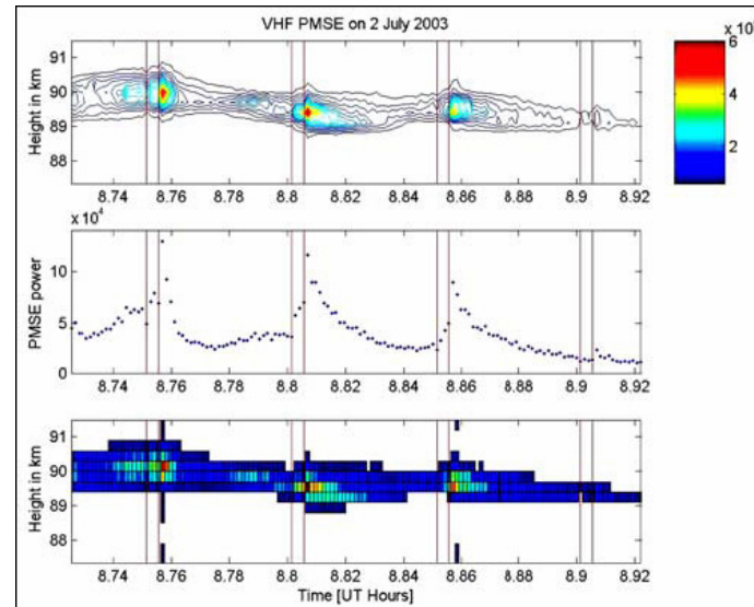
Figure 1: PMSE echo strength showing an overshoot immediately after switch the 3s long heater pulse off. HF on is shown by the vertical lines. The bottom panel shows the raw data, corrected for radar transmitter power, while the upper panel shows the same data but now smoothed. The relative intensity scale is the same for both panels, and the background noise on this linear scale is at approximately 2500. The middle panel shows the sum of the three highest intensities at each time sample and is a measure of the total PMSE intensity as a function of time. Taken from [18].
