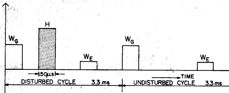
(b) Conventional Cross Modulation
