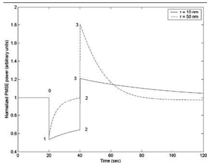
Figure 2: Model calculations showing how the shape of the overshoot phenomenon depends on particle size. HF is on from 20 to 40 s and the amplitude from 0 to 1 depends on the electron heating. Taken from [18].
