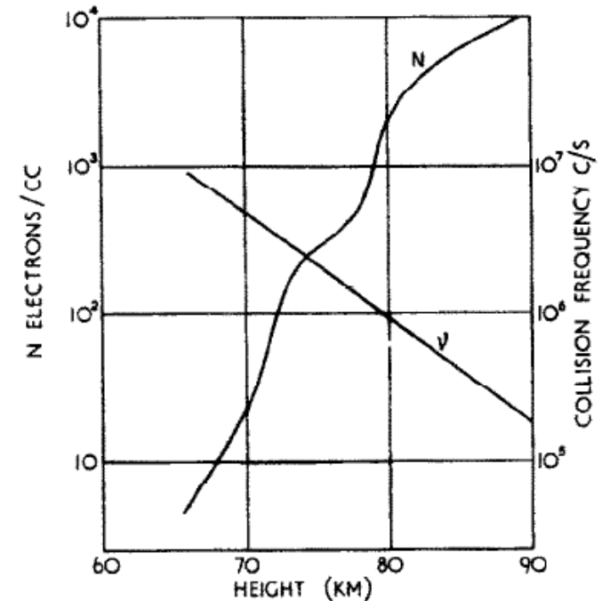
Fig. 4. Collision frequencies and electron densities derived from the experimental data of Fig. 3.
