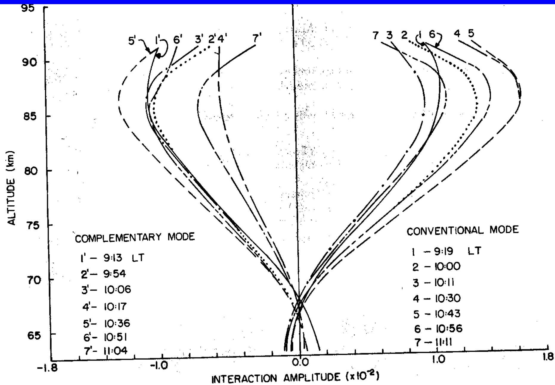
Fig. 2. Observed amplitude cross modulation for conventional and complementary modes.
