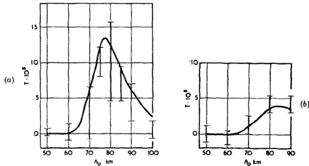
Fig. 3. Mean values and standard deviations of records for different values of h_o . Fig. 3a represents records taken with extraordinary polarization, Fig. 3b records taken with ordinary polarization of the disturbing wave. The lengths of the vertical lines are equal to twice the standard deviation, their midpoints indicate mean values. The solid theoretical curve corresponds to the conditions of Fig. 4.
