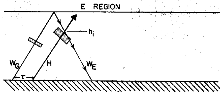
(a) Geometry of Conventional Cross Modulation
