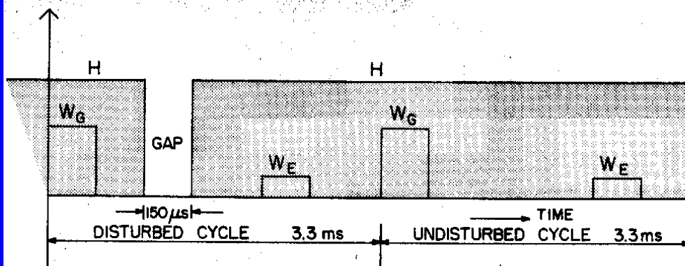
(c) Complementary Cross Modulation
