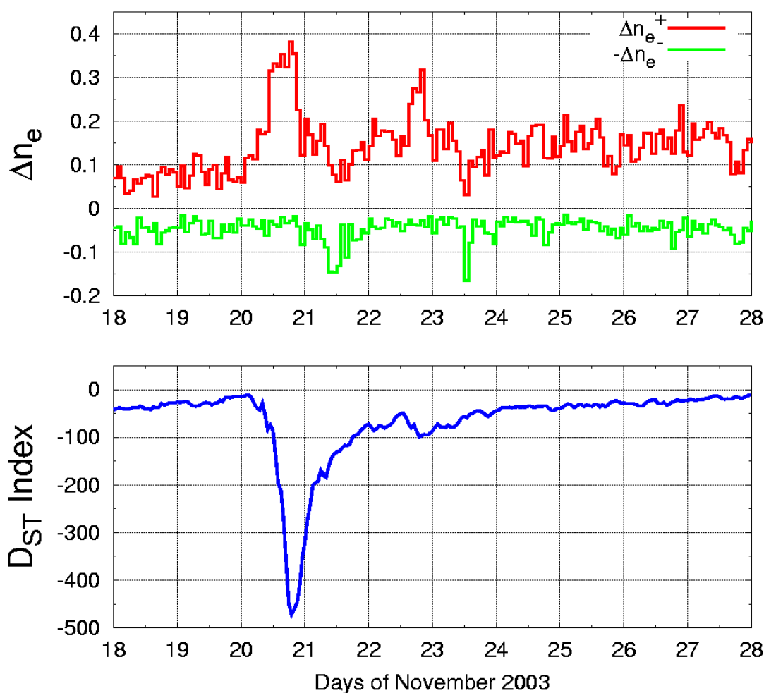
Fig. 14: Comparison of positive and negative deviation counts of the electron density values that exceed a certain threshold value ( |\Delta n_e| > 50\% ) from corresponding means with the geomagnetic D_{st} index ( http://swdcdb.kugi.kyoto-u.ac.jp/dstdir/ ).
