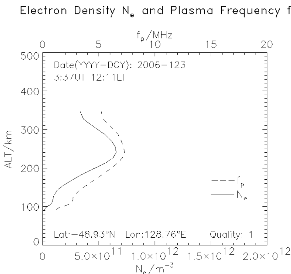
Fig. 5 Data product sample showing the IRO retrieval of the SWACI service.
