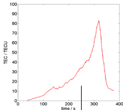
CHAMP IRO data - 52.82°N; 164.73°E, 12:30 UT
