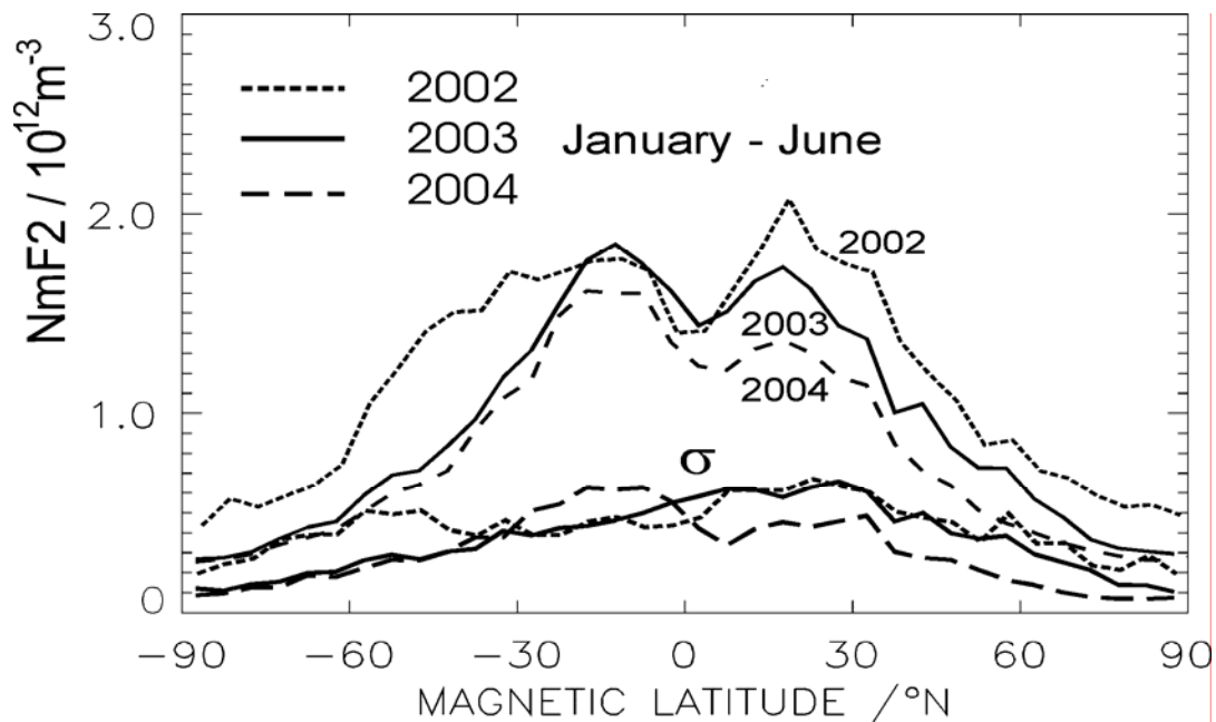
Fig. 8: Latitudinal dependency of the day-time (08:00-16:00 LT) F2 layer peak electron density NmF2 as seen in the CHAMP IRO data at three years 2002-2004 for all longitudes. The corresponding standard deviation \sigma is given at the bottom of the figure.
