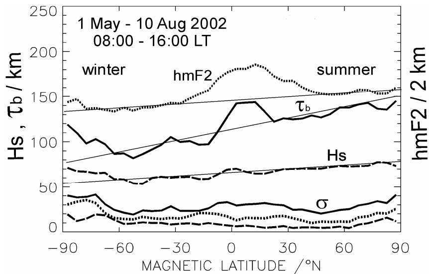
Fig. 10: Latitudinal dependence of the peak density height hmF2 and shape parameters such as bottomside slab thickness \tau_b and the topside scale height H_s at 425 km height measured at daytime in Northern summer. The corresponding standard deviation \sigma of all three parameters is given at the bottom of the figure.
