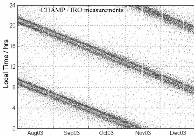
Fig. 4 Local time sector of ionospheric radio occultation measurements during months August – December 2003.
