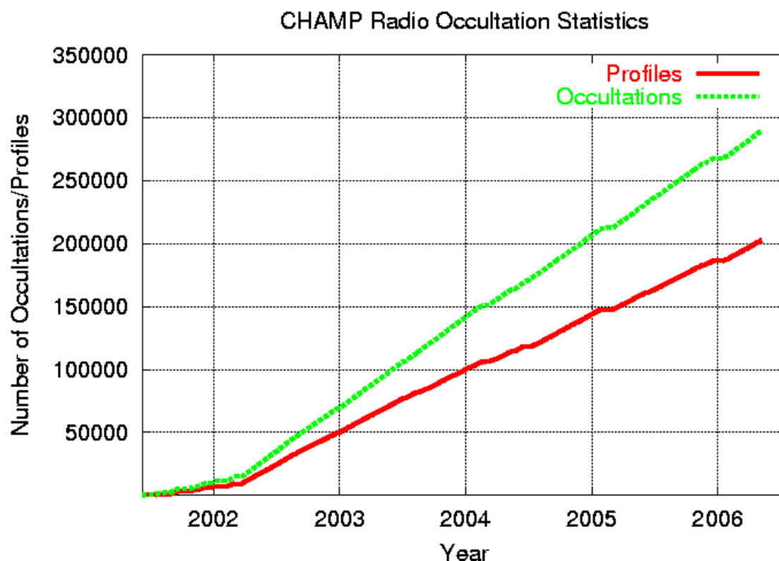
Fig. 2 Number of IRO measurements and retrieved vertical electron density profiles from 11 April 2001 until end of April 2006.
