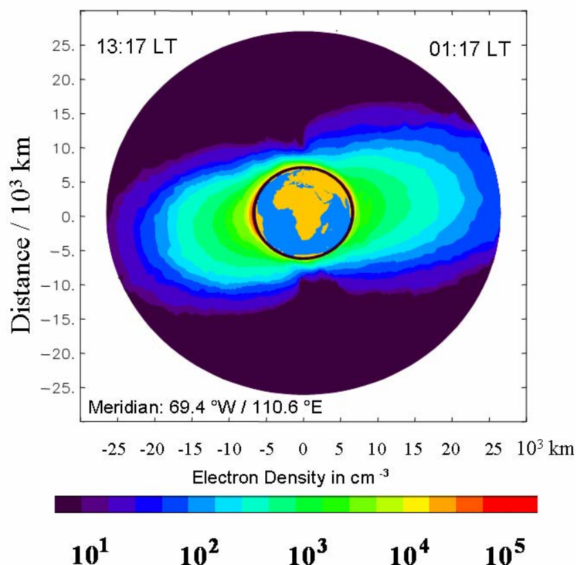
Fig. 7: Reconstruction of the electron density distribution of the topside ionosphere based on GPS data received onboard CHAMP. The reconstruction is based on medians obtained for 21:00 UT over 10 consecutive days in August 2005. Thus, the right side shows the ionosphere/plasmasphere shortly after midnight whereas the left side represents ionosphere shortly after noon.
