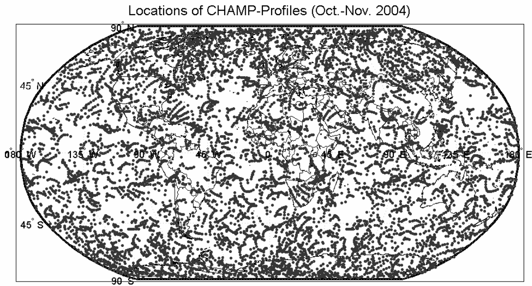
Fig. 3 Locations of retrieved radio occultation profiles during two months (October – November 2004).
