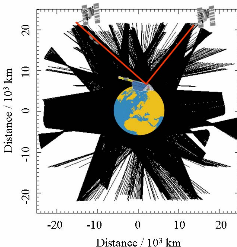
Fig. 6: Illustration of the topside radio link distribution in the CHAMP orbit plane to the visible GPS satellites during one satellite revolution.
