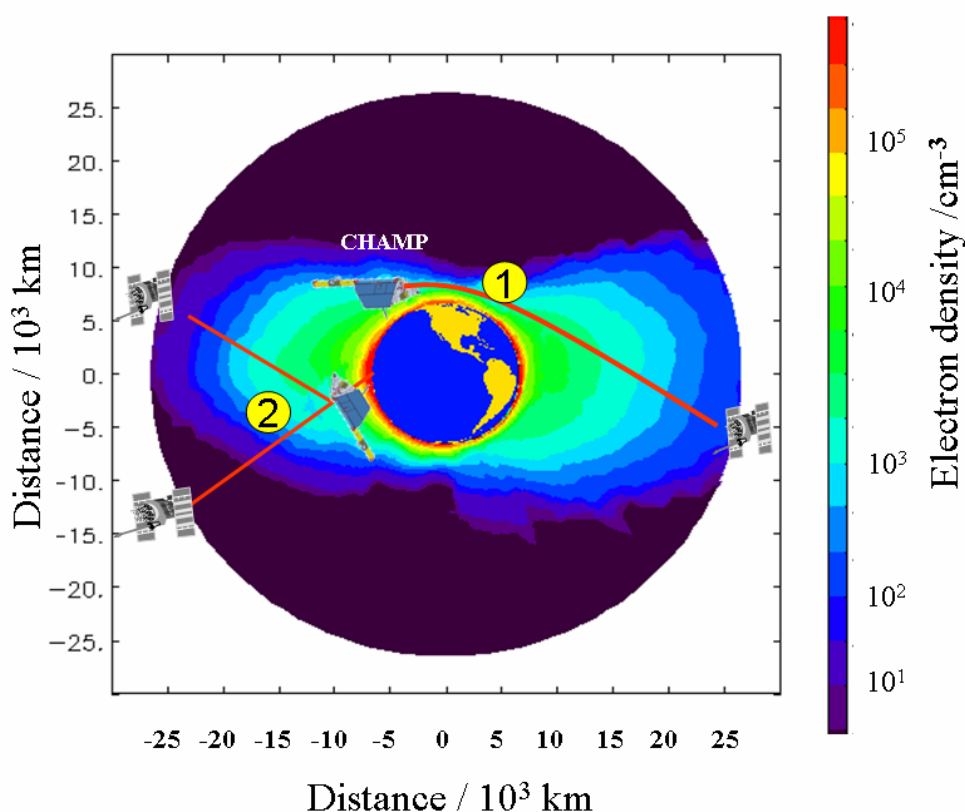
Fig. 1: Illustration of GPS measurement techniques used onboard CHAMP for sounding the ionosphere. (1): Ionospheric radio occultation (IRO) measurements in the limb sounding mode. (2): Use of 0.1 Hz sampled GPS navigation data from the zenith viewing antenna.
