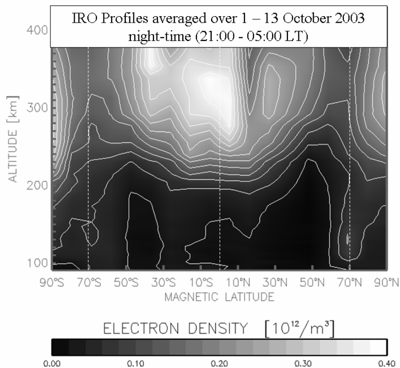
Fig. 11: Imaging of the average vertical ionization structure constructed from all IRO profiles obtained during the first 13 days in October 2003 between 21:00 and 05:00 LT. Marked are geomagnetic latitudes at 70° and at 0°.
