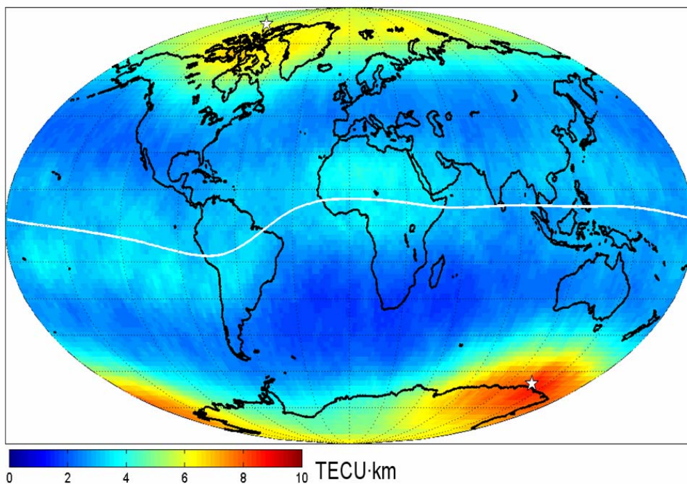
Fig. 12: Global distribution of the occurrence of ionospheric irregularities (characteristic scale length about 15-30 km) detected in IRO CHAMP data from March 2002 – February 2006. Geomagnetic poles are marked by asterisks, the magnetic equator by a full line.
