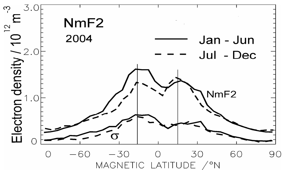
Fig. 9: Latitudinal dependence of the peak electron density NmF2 summarizing all measurements obtained in 2004 in the first and second half years at daytime (08:00 -16:00 LT) for all longitudes. The crest locations are marked at about \pm 15^\circ magnetic latitude and the standard deviation \sigma is given at the bottom of the figure.
