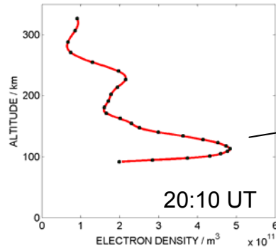
CHAMP Profile 2003 DOY: 302, 22:58:12 LT Lat. [°N]: -68.23, Lon. [°E]: 41.54
