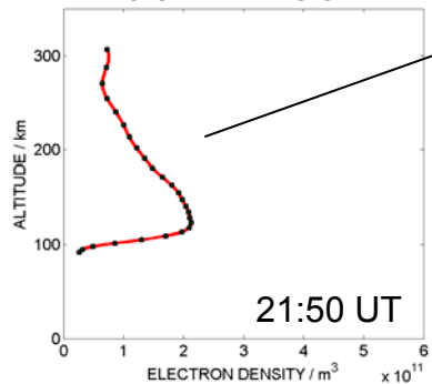
CHAMP Profile 2003 DOY: 302, 0:44:24 LT Lat. [°N]: -51.73, Lon. [°E]: 43.63
