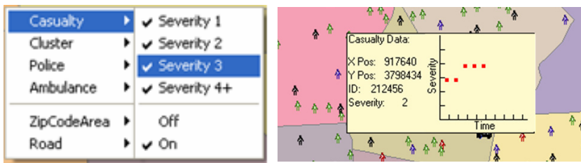
Figure 10. Fast data manipulation and identification: resource context menu (left), and pop-up window for object identification and the visualization of its trend (right).
