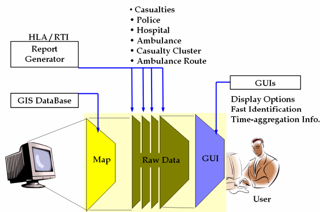
Figure 3. Data layers of the software architecture
