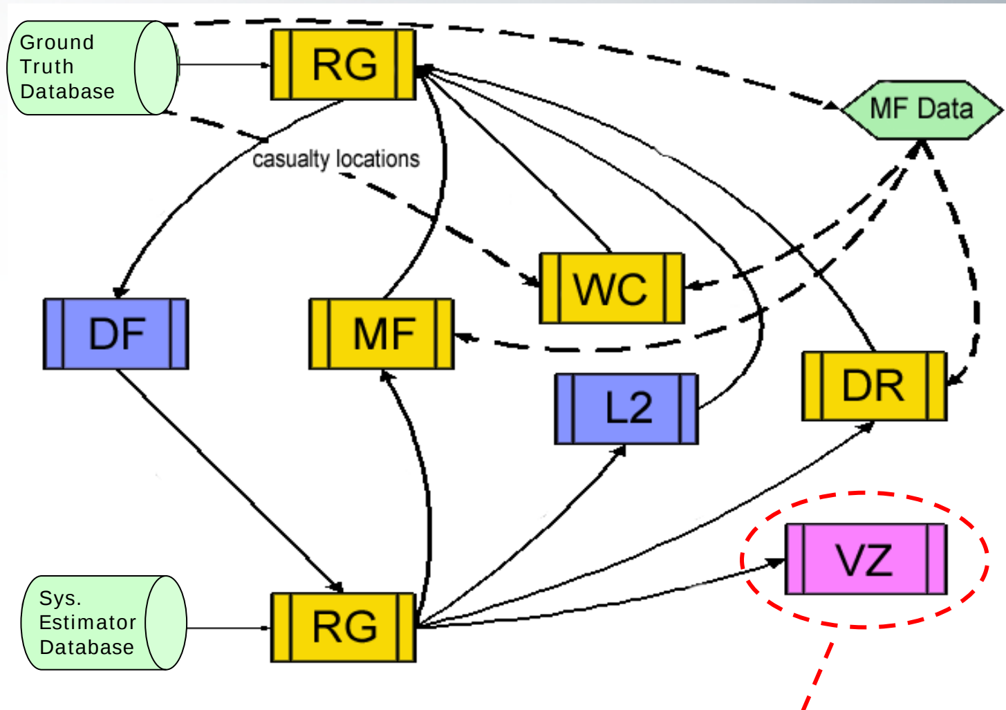
Location of Visualization Federate in HLA/RTI Interface
