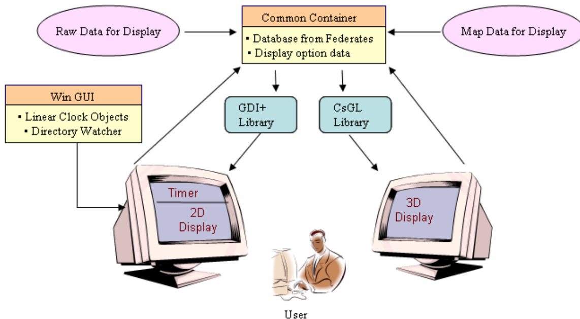
Figure 7. Integrated simulation architecture for multiple and different display of 2D and 3D.
