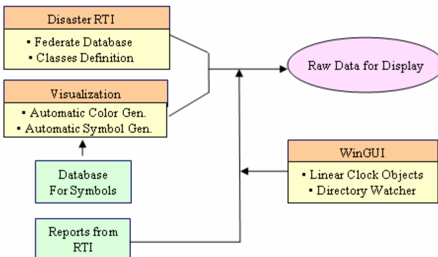
Figure 5. Pipelines to Report Data Generation
