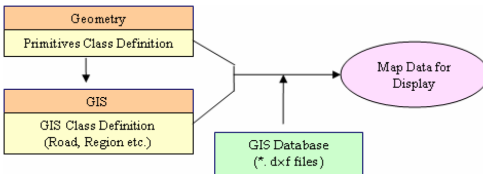
Figure 4. Pipelines to Map Data Generation.
