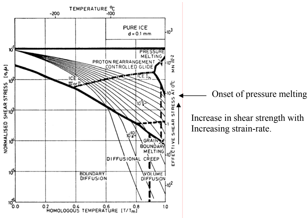
Figure 10. Deformation-mechanism map for ice. Note that increasing the strain-rate by 5 orders of magnitude near 0^{\circ}\text{C} increases the shear strength (effective shear stress) by a factor of 10. This increase in strength is limited by pressure melting that occurs at an effective shear stress of about 10 MPa. (From Frost and Ashby, 1982).
