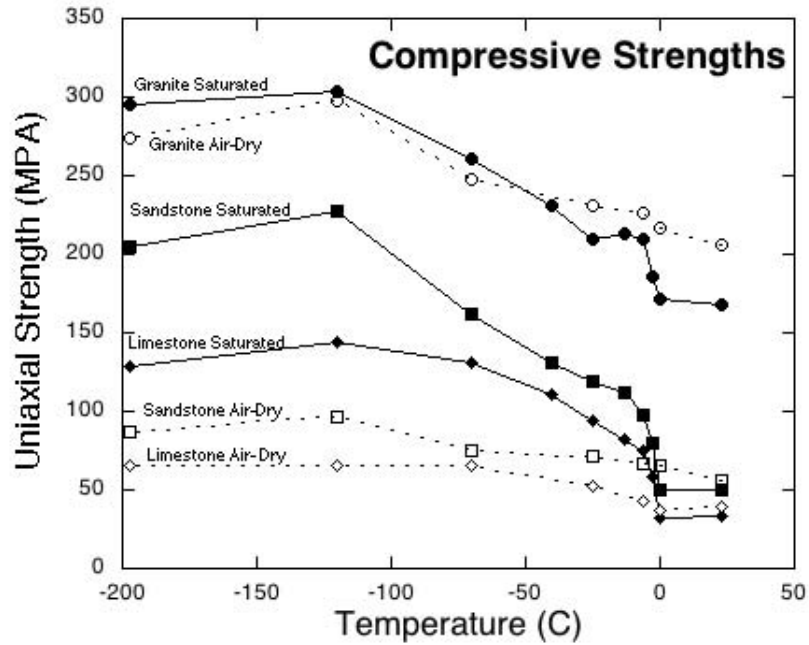
Figure 4. Strength of granite, limestone, and sandstone in uniaxial compression at low temperatures from Mellor (1973). Note that only in granite are the strengths of saturated and air-dry samples nearly the same at all temperatures.
