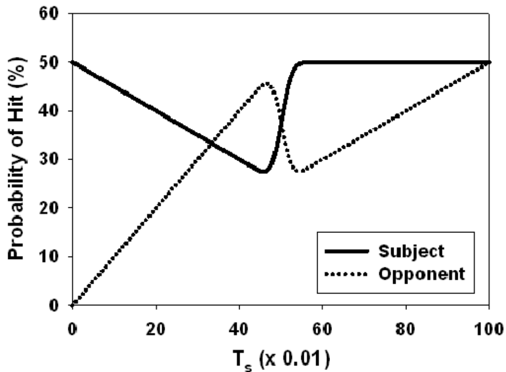
Figure 4. Mean probabilities of being hit as a function of the subject's shooting time ( T_s ) for scenario #2 (opponent shooting preference of \mu = 0.50 and \sigma = 0.02 ).
