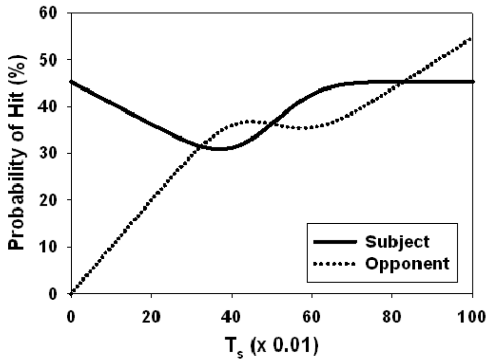
Figure 5. Mean probabilities of being hit as a function of the subject's shooting time ( T_s ) for scenario #3 (opponent shooting preference of \mu = 0.45 and \sigma = 0.10 ).
