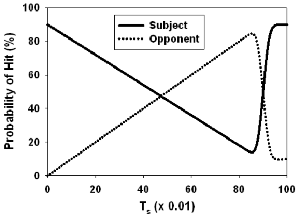
Figure 3. Mean probabilities of being hit as a function of the subject's shooting time ( T_s ) for scenario #1 (opponent shooting preference of \mu = 0.90 and \sigma = 0.02 ).
