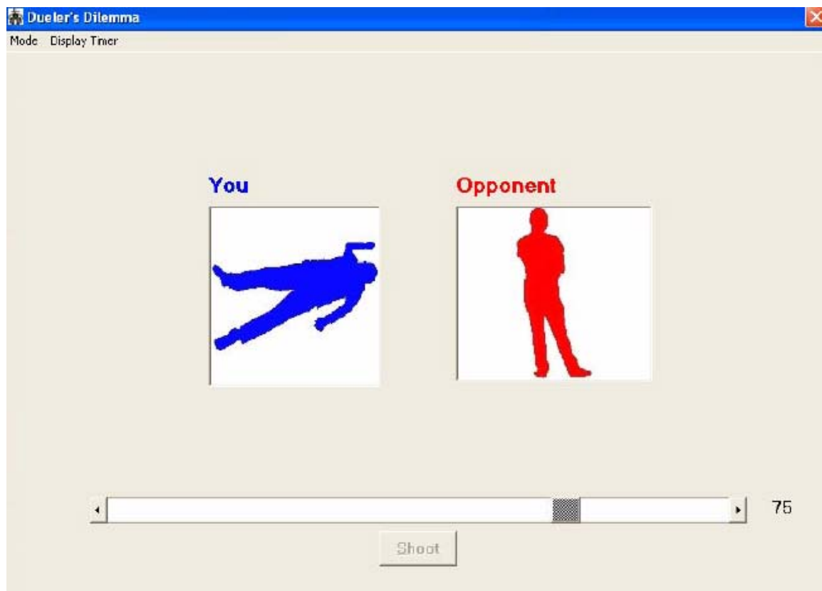
Figure 6. Example display of a possible discrete outcome when the subject shoots at a scaled time of 75 (i.e., T_s = 0.75 ).
