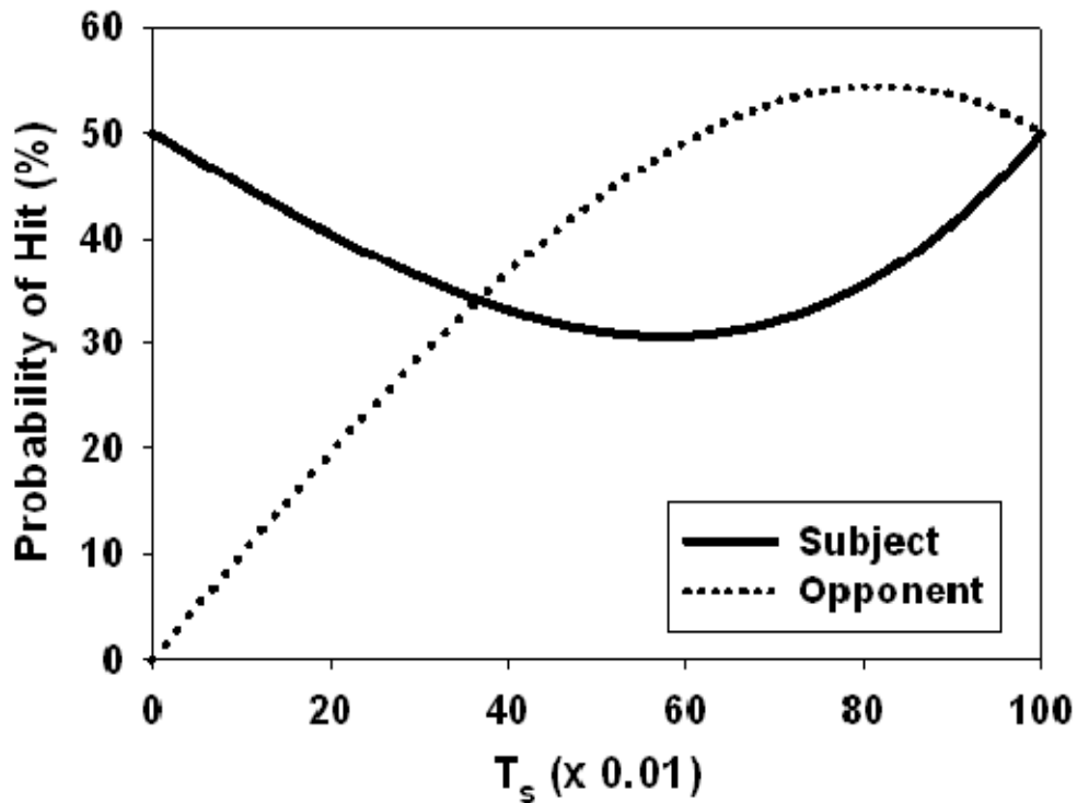
Figure 2. Mean probabilities of being hit as a function of the subject's shooting time ( T_s ) for completely randomized opponent's shooting times. The zone of advantage begins at T_s = 0.37 and continues to the right.
