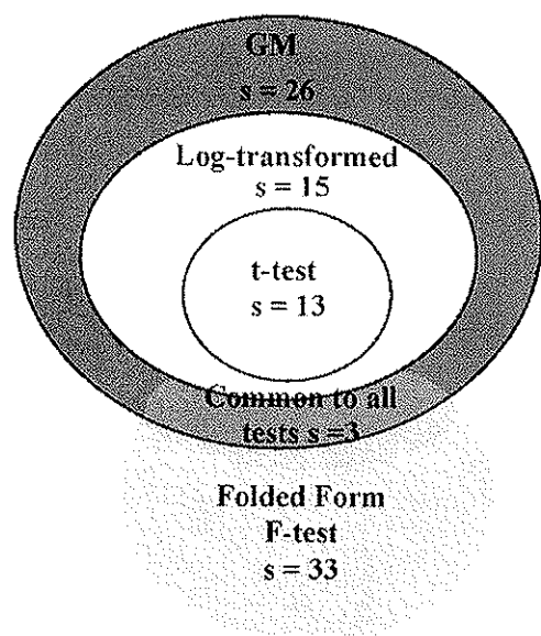
Figure 6. Nested collection of significant spots. The GM procedure found the same spots as the traditional t-test as well as those found from testing on the log-transformed data. The number of unique spots using the Folded Form F-test ( s = 33 ) are demonstrated by the green circle. Three spots were found to be significant regardless of testing method.
