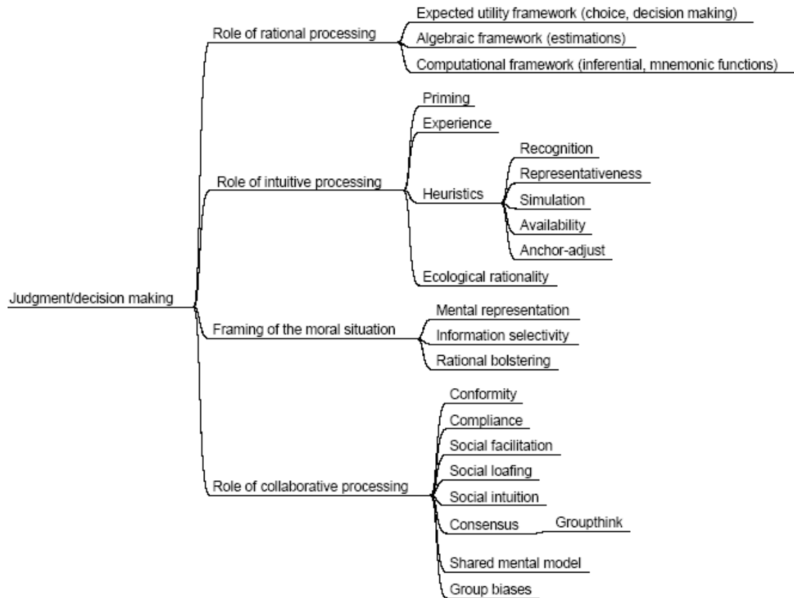
Figure 5. Judgment/decision-making
