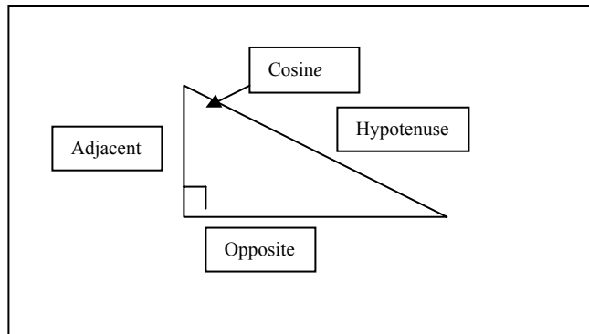
Figure 5. Cosine = Adjacent/Hypotenuse
