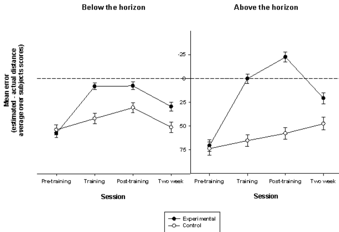
Figure 11. The experimental (solid dots) and control group's (open dot) mean error scores, in metres, plotted by session (pre-training, training, post-training and two week post training) both above and below the horizon. The dotted line at zero represents a perfect score. The experimental group does not depart significantly from zero during the training and post training sessions (unit is metres). The control group did not show significant improvement in either case.
