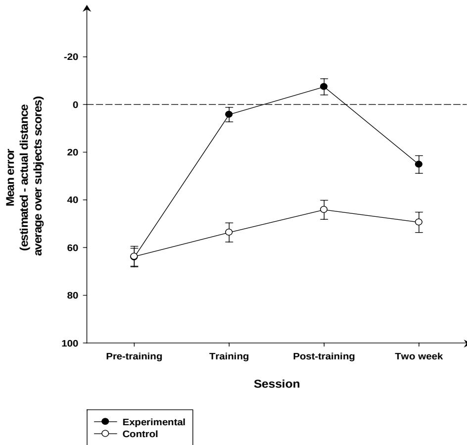
Figure 12. The experimental (solid dots) and control group's (open dot) mean error scores, in metres, plotted by session (pre-training, training, post-training and two week post training). Experimental group is significantly more accurate than the control group during and after the training session. The experimental group's training, post-training and two-week post-training sessions are significantly more accurate than its pre-training session (unit is metres).
