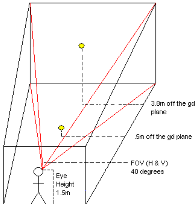
Figure 10. 3-D diagram of the simulated environment using perspective projection. Shaded dots indicate flashes.
