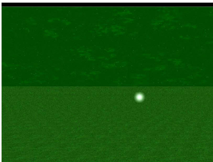
Figure 7. Below the horizon flash
