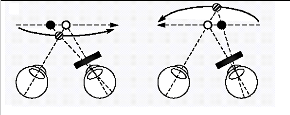
Figure 4. The Pulfrich effect. An object oscillating back and fourth appears to traverse in an elliptical path as the result of a delay in one eye. Reproduced from “Joint-encoding of motion and depth by visual cortical neurons: neural basis of the Pulfrich effect” by A. Anzai, I. Ohzawa, and R.D. Freeman, 2001, Nature Neuroscience , 4(5).
