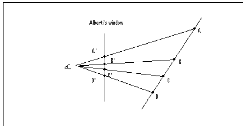
Figure 2. Alberti’s window illustrates the concept of invariance, that is, the same constant is derived from A'B'C'D and A'B'C'D' ( (AB \cdot CD) / (AD \cdot CB) = (A'B' \cdot C'D') / (A'D' \cdot C'B') ). Reproduced from “Perception with an eye for motion” by J.E. Cutting, 1986, Cambridge, MA: MIT Press.
