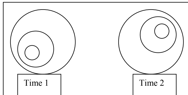
Figure 1. The stereokinetic effect demonstrates a transformation in perception over time from 2-D circles rotating around each other to 3-D cones wobbling. Reprinted from "The logic of perception" by I. Rock, 1983, Cambridge, MA: MIT Press.
