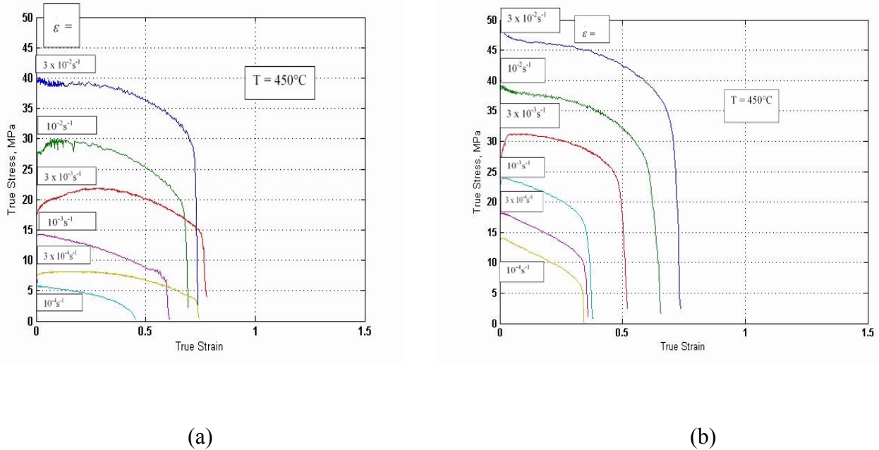
Figure 13. Stress Strain curves for tensile tests done at 450°C for G1, HB material rolled to 74% reduction at (a) RT and (b) 300°C.
