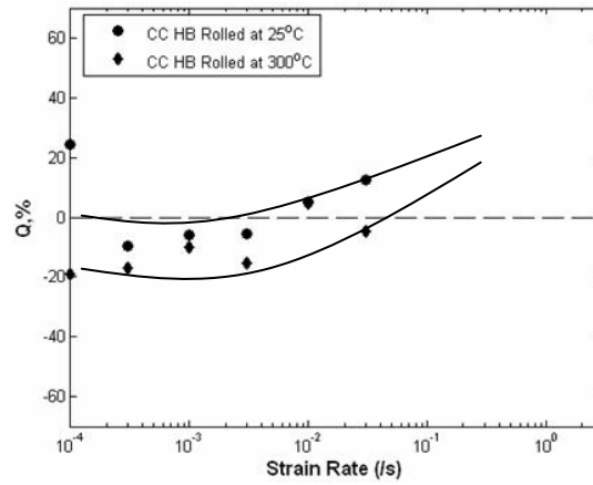
Figure 14. (a) \sigma_{0.1} , (b) Ductility and (c) Q\% vs. \dot{\epsilon} rate for HB, G1 material rolled at RT and 300°C to 74% reduction and tested at various strain rates at 450°C.
