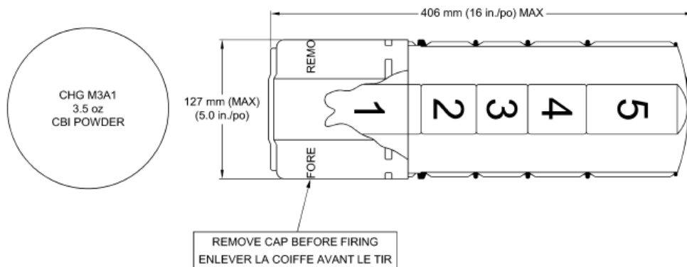
Figure 2. M1 propellant charge for the 155 mm
