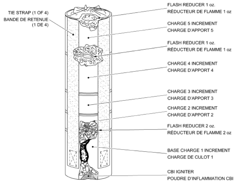
Figure 3. Propellant bags within the M1 charge
