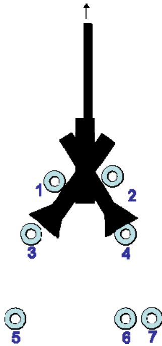
Figure 5. Positions of the gunners (blue circles) around the M777 105 mm howitzer
