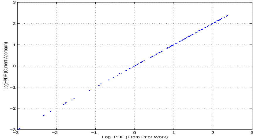
Figure 1: Comparison of Saddlepoint Approximation from previous work (x-axis) with method of this section for cyclic ACF estimates. The largest difference was .021
