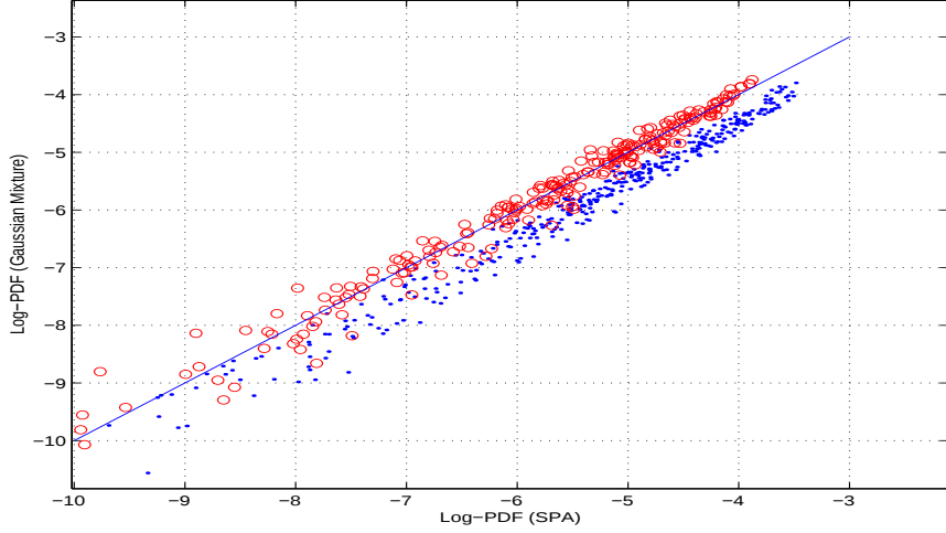
Figure 2: Comparison of Saddlepoint Approximation from reference with a Gaussian mixture approximation. Dots are without first-order correction term, circles with correction term.
