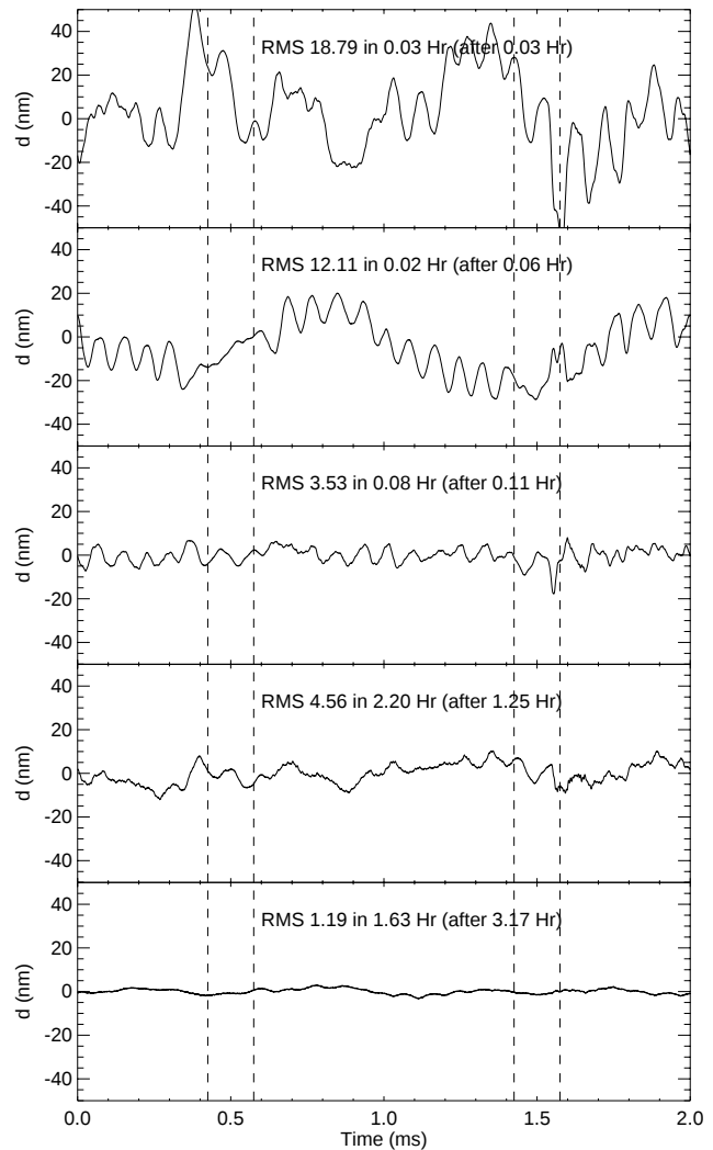
Figure 8. Change in mean stroke between consecutive measurement of the stroke. In each panel is also listed the RMS of this variation over the used range of the stroke.
