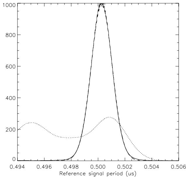
Figure 2. Histogram of the reference time (solid), and of the unknown time (dotted) for test FDL_2005_04_12_1232. A Gaussian fit to the reference time distribution is plotted as a dashed curve.
