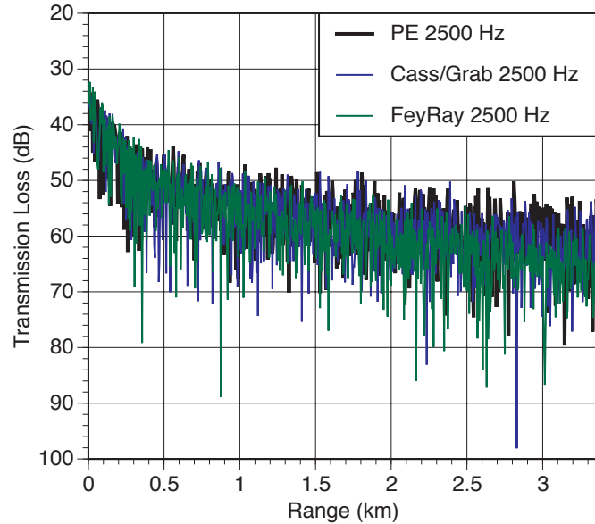
Figure 29 . Plot of transmission loss predictions for PE, FeyRay, and GRAB for ASA wedge problem at a frequency of 2500.
