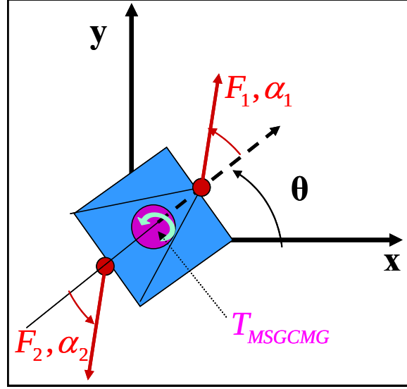
Figure 39. Spacecraft Simulator Dynamics Schematic
