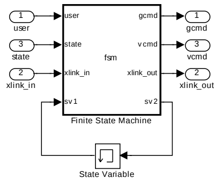
Figure 39. Onboard Autonomy SIMULINK model
