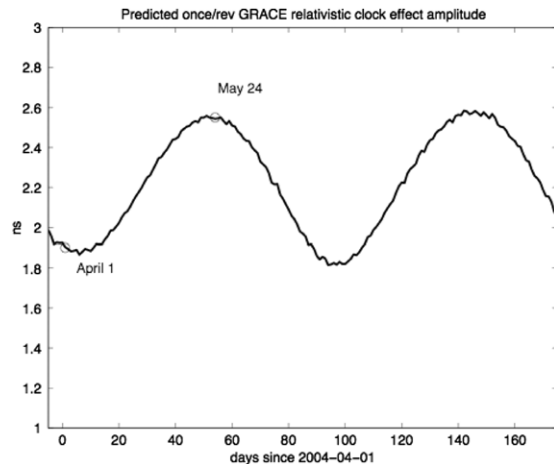
Figure 1. Amplitude of the once/rev relativistic clock effect predicted for the GRACE satellites using equation (1).
