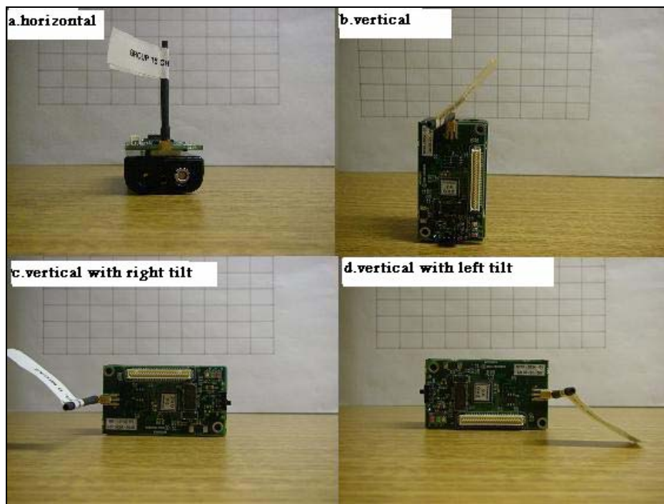
Figure 12. Multiple Test Position for the MICAz Mote, (a) Horizontal Cut Plane, (b) Vertical Cut Plane, (c) Vertical Cut Plane with Right Tilt, and (d) Vertical Cut Plane with Left Tilt.
