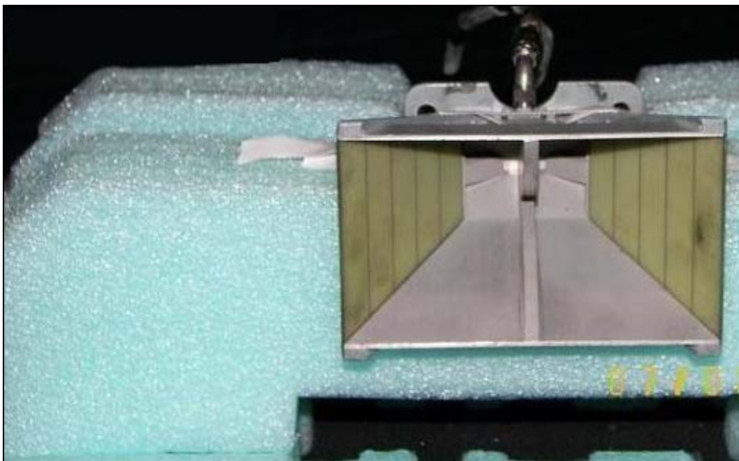
Figure 23. The AEL Pyramidal Horn Antenna at the Anechoic Chamber Gain Measurement.
