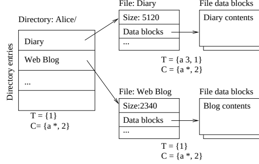
Figure 4: File and directory labels. User Alice owns a publicly readable directory Alice , a publicly readable file Web Blog , and a private file Diary . Only processes with privilege tag a* may modify her files.
