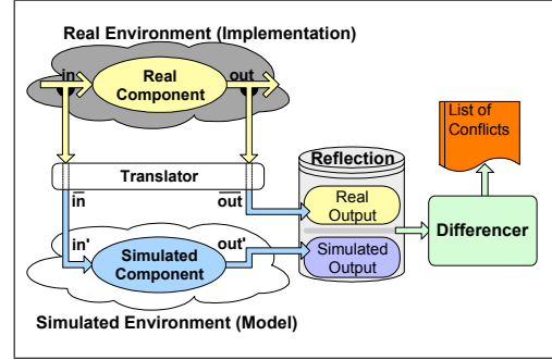
Figure 4. Architectural Differencing
