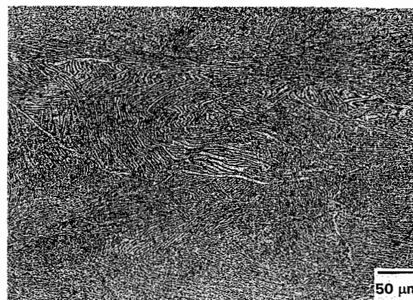
Fig. 10. Microstructure of specimen deformed at 950^\circ\text{C} and 10 \text{ s}^{-1} . The compression axis is vertical.
