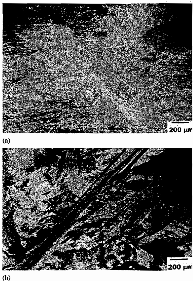
Fig. 9 Microstructures obtained on Ti-6Al-4V specimens deformed at 750^\circ\text{C} and 100 \text{ s}^{-1} : (a) coarser grained material and (b) coarse grained material. The compression axis is vertical
