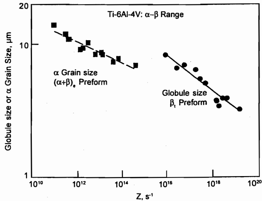
Figure 6: Variation of globule size ( \beta_i preform) and \alpha grain size ( ((\alpha+\beta)_e preform) with Zener-Hollomon ( Z ) parameter in the \alpha - \beta range of Ti-6Al-4V.
