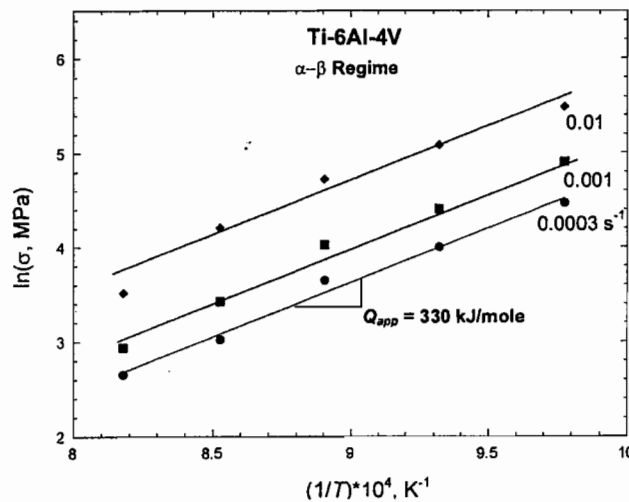
Fig. 4. Arrhenius plot showing the variation of flow stress with inverse of temperature in the \alpha - \beta regime of Ti-6Al-4V at different strain rates.
