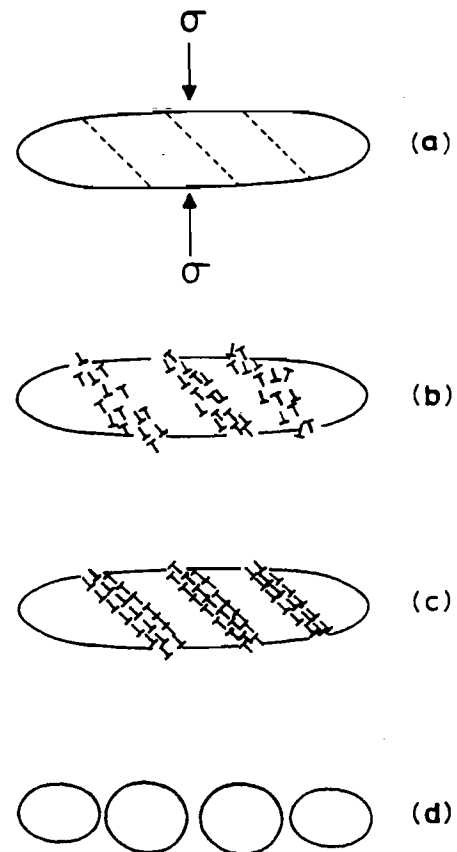
Fig. 7. Schematic illustrating the steps of globularization process.
