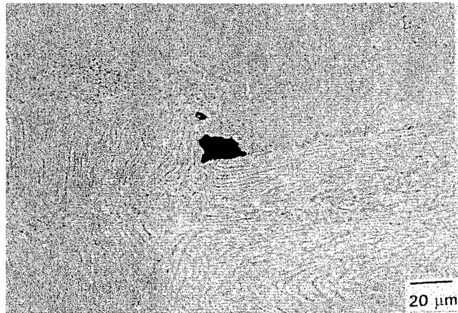
Figure 10: Microstructure obtained in a Ti-6Al-4V \beta_1 preform specimen deformed at 750°C and 0.001 s -1 . The compression axis is vertical.
