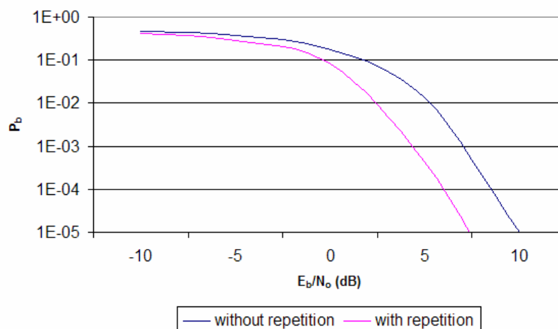
Figure 37. Comparison of CSK BER with and without repetition code.
