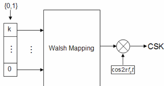
Figure 30. CSK modulator.
