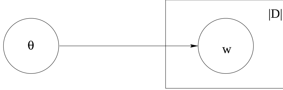
Figure 1.1. Graphical representation of the Multinomial distribution
