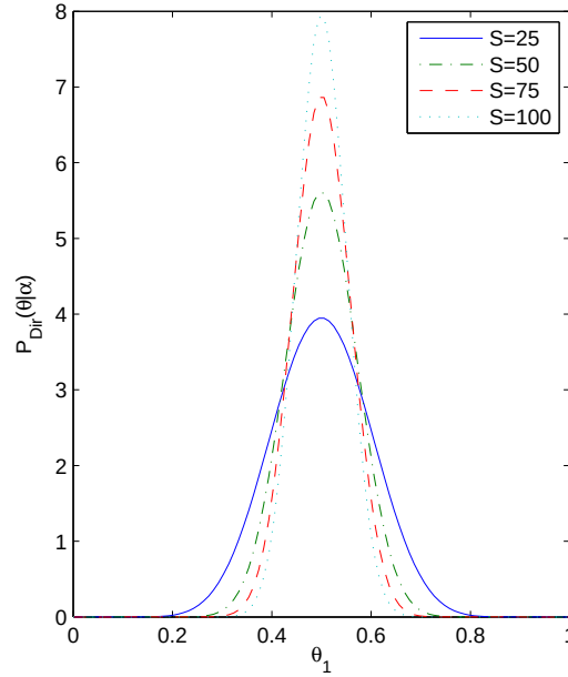
Figure 5.1. Dirichlet distribution has lower variance for higher values of precision S
