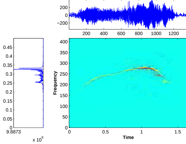
Figure 9: A whale sound.
