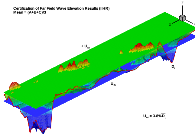
Figure B9 3D surface of difference D_i of wave elevation results ( Fr=0.28 )
