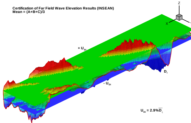
Certification of Far Field Wave Elevation Results (IIHR) Mean = (A+B+C)/3
