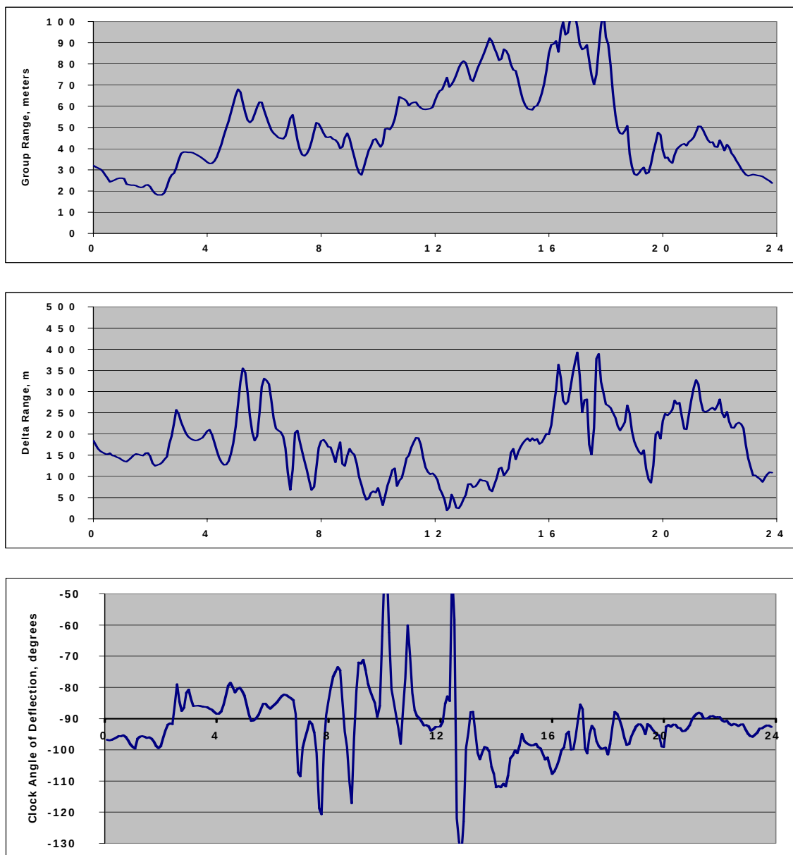
Figure 7: Upper plot – group delay range error. Center Plot – magnitude of the deflection vector. Lower plot – direction of deflection vector. (5 degree elevation angle results - October 14, 2003)
