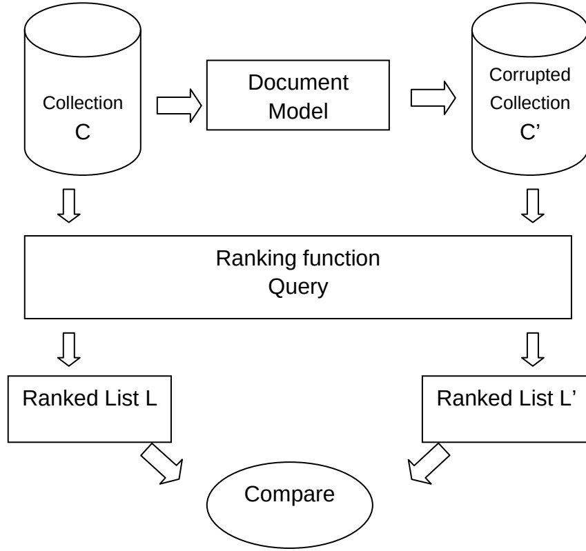
Figure 3.3 : Robustness Score Calculation
