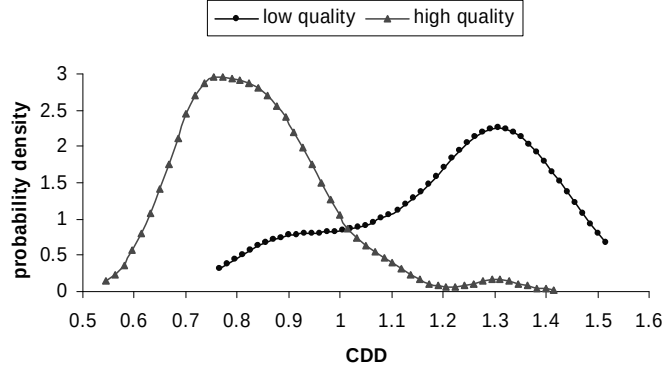
Figure 6.1: Distribution of CDD values for low and high quality documents.
