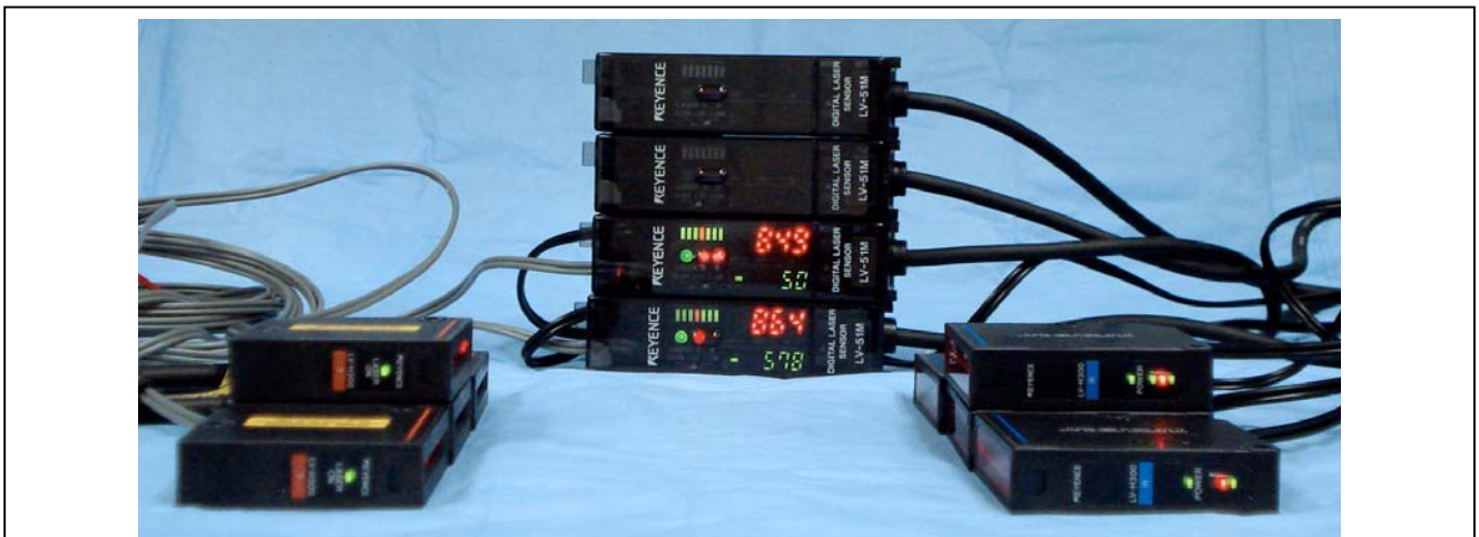
Fig. 7 Bench-top test of ribbon lasers ( Keyence ). Four 4cm wide lasers transmitters are shown at right opposite receivers at left (model LV-H300). Amplifiers with signal readout are in stacked in the middle (model LV-51M).
