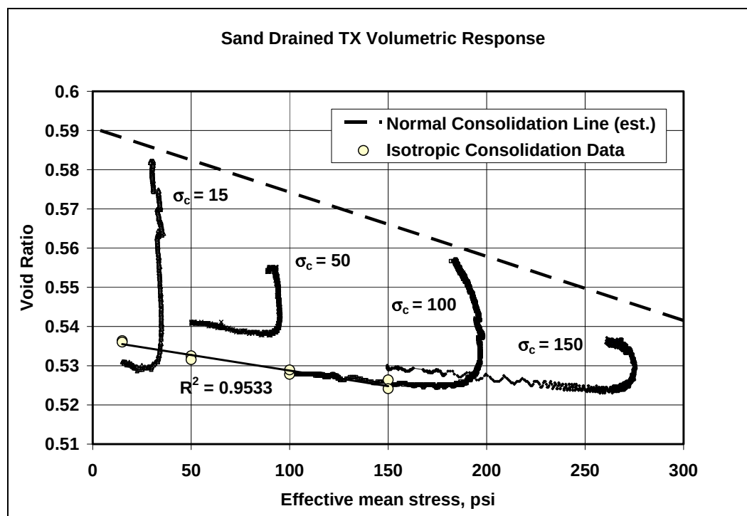
Figure 12. Drained and undrained isotropic and drained hydrostatic response for SP sand.
