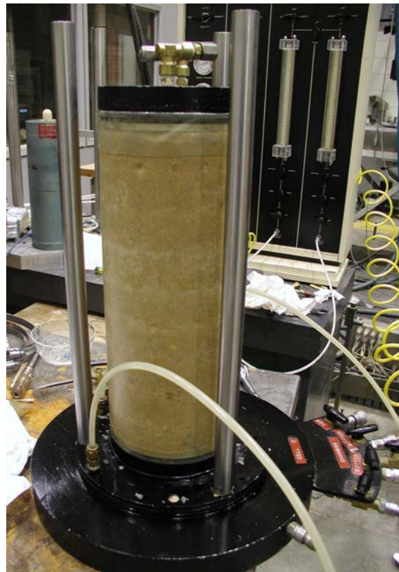
Figure 8. Triaxial specimen of SP sand after compaction.
