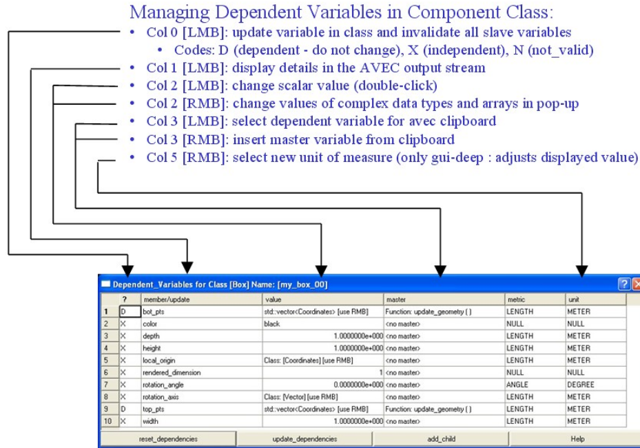
Figure 10. Examine Component Pane
