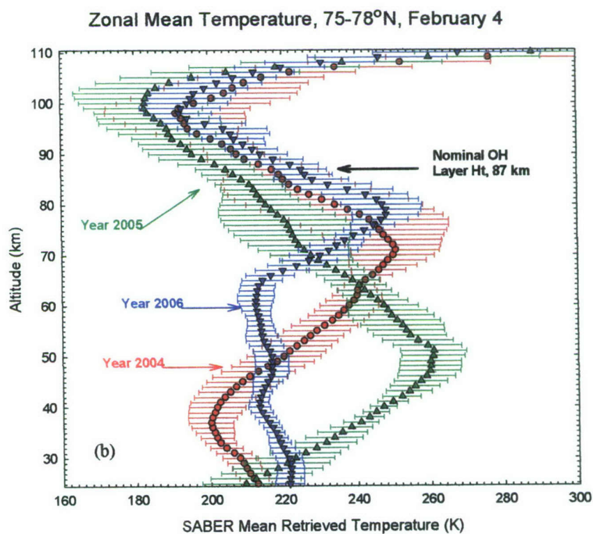
Figure 6. Comparison of zonal-mean retrieved temperature in the latitude range 75-78°N, for two days in boreal winters 2004 (red), 2005 (green), and 2006 (blue). (a) January 19; (b) February 4. Error bars are 1-sigma.
