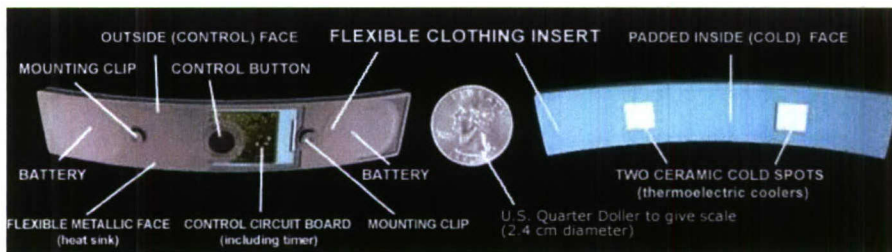
Figure 19. It's Kool™ Personal Cooling Device (It's Kool™, 2006)
