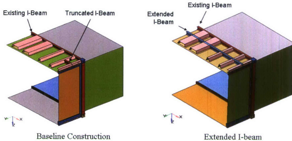
Figure 20. Floor Stiffening Concept Using Extended Subframe I-Beams
