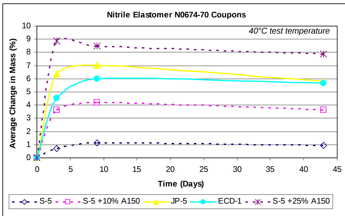
Figure E-5. Average Mass Change (%) Over Time for Nitrile Elastomer N0674-70 Coupons
