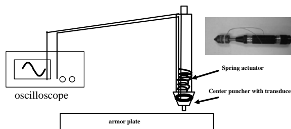
Fig. 16: Hand-held "impact method" prototype
