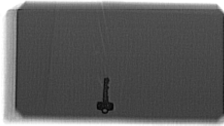
Fig. 6: X-ray image of a VBASS plate with a hairline crack
