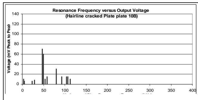
Fig. 9: PZT transducer voltage vs. frequency for the hairline cracked plate
