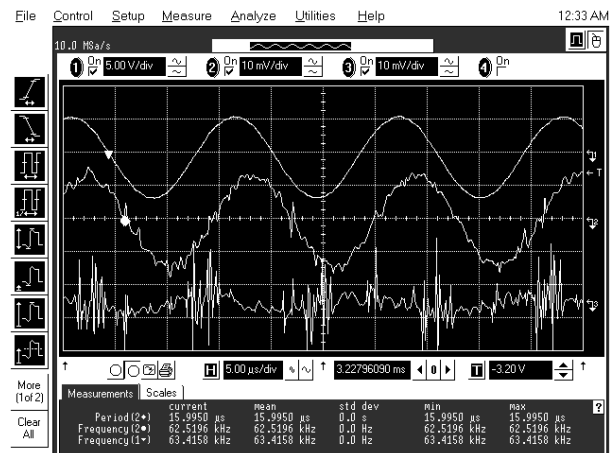
Fig. 5: Oscillogram of input and output voltages
