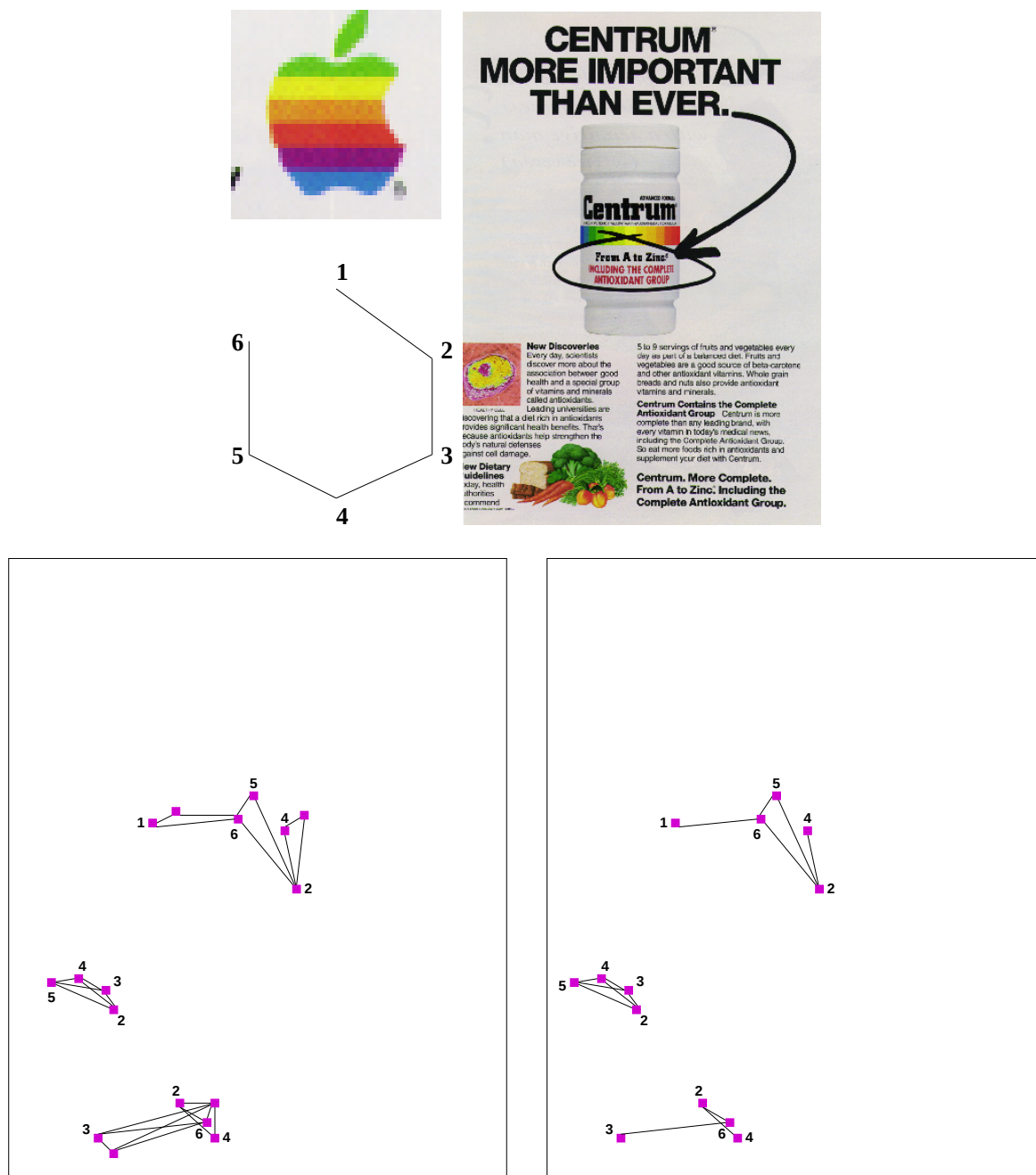
Figure 3.12. Example of reduction of SPGs after phase 1 in a false match: (top left) query and query graph; (top right) false match retrieved after phase 1; (bottom left) SPG stored offline; (bottom right) reduced SPG which did not match the query graph (hence this image is deleted by phase 2)
