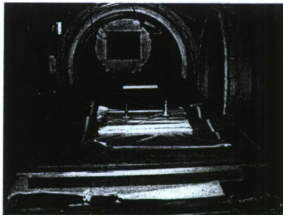
Figure 5 – Neat resin specimens (background) and EMC laminate (foreground) being placed in the autoclave for cure.
