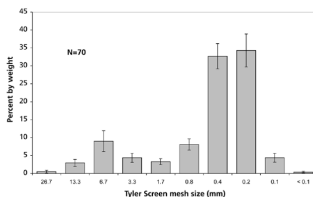
Figure 14. Puget Sound sand lance spawning substrate grain-size spectrum.
