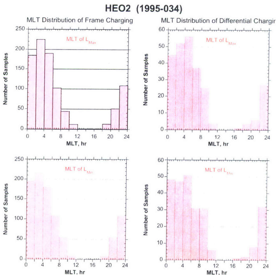
Figure 6. MLT Distribution of HEO2 frame charging (left panels) and differential charging (right panels) for L_{MAX} (upper panels) and L_{MIN} (lower panels).
